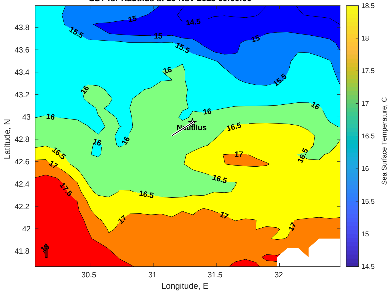
SST for Nautilus at 16-Nov-2025 00:00:00
