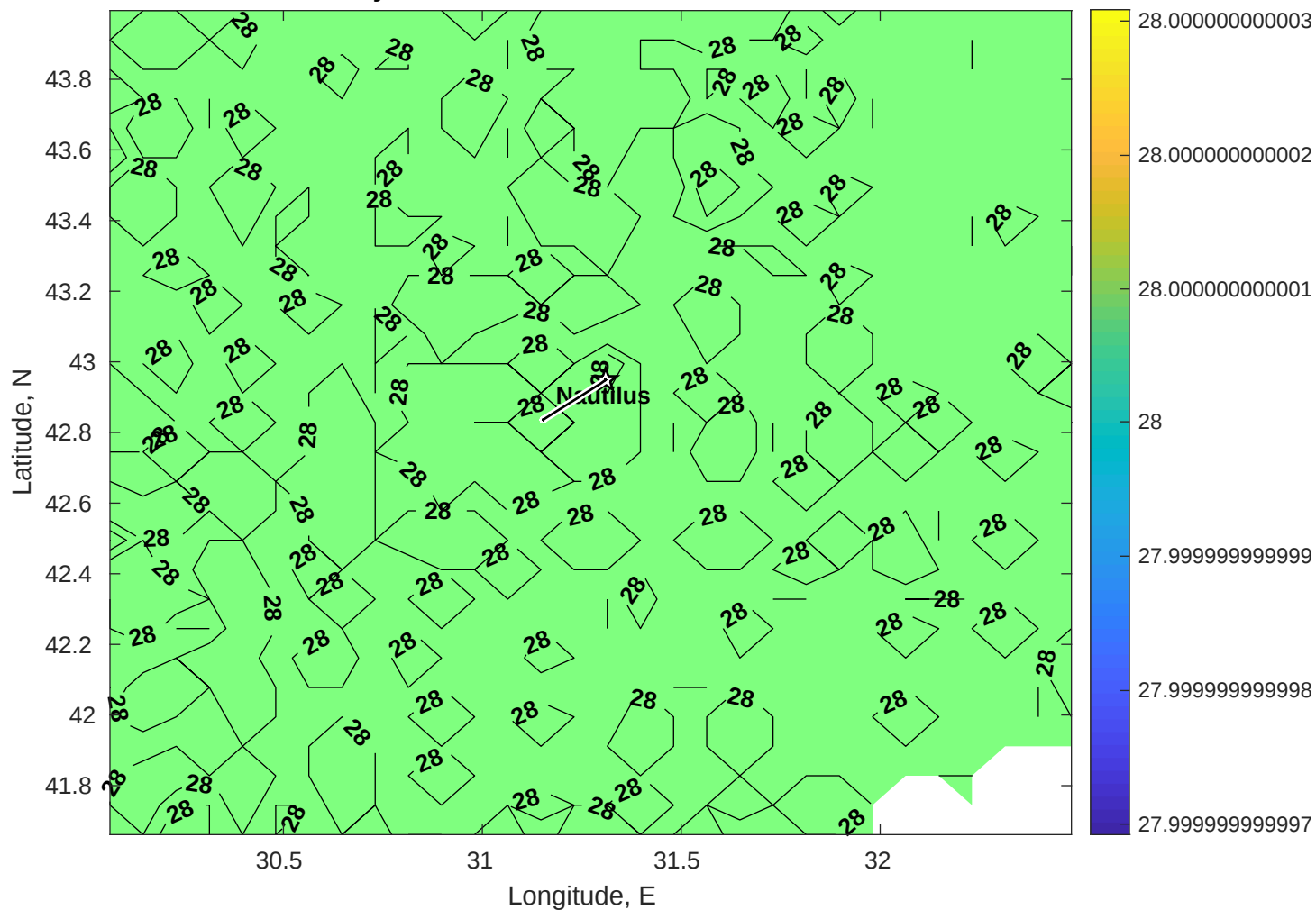
Surface Salinity for Nautilus at 16-Nov-2025 00:00:00
