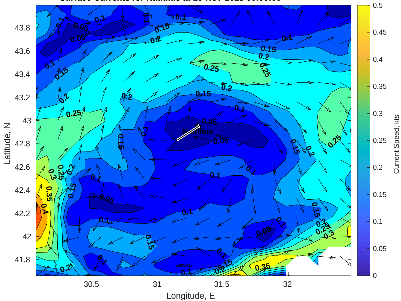
Surface Currents for Nautilus at 16-Nov-2025 00:00:00
