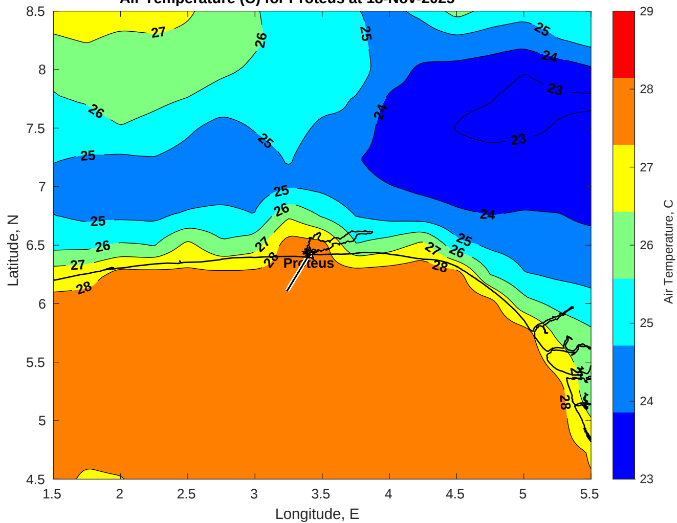
Air Temperature (C) for Proteus at 18-Nov-2025
