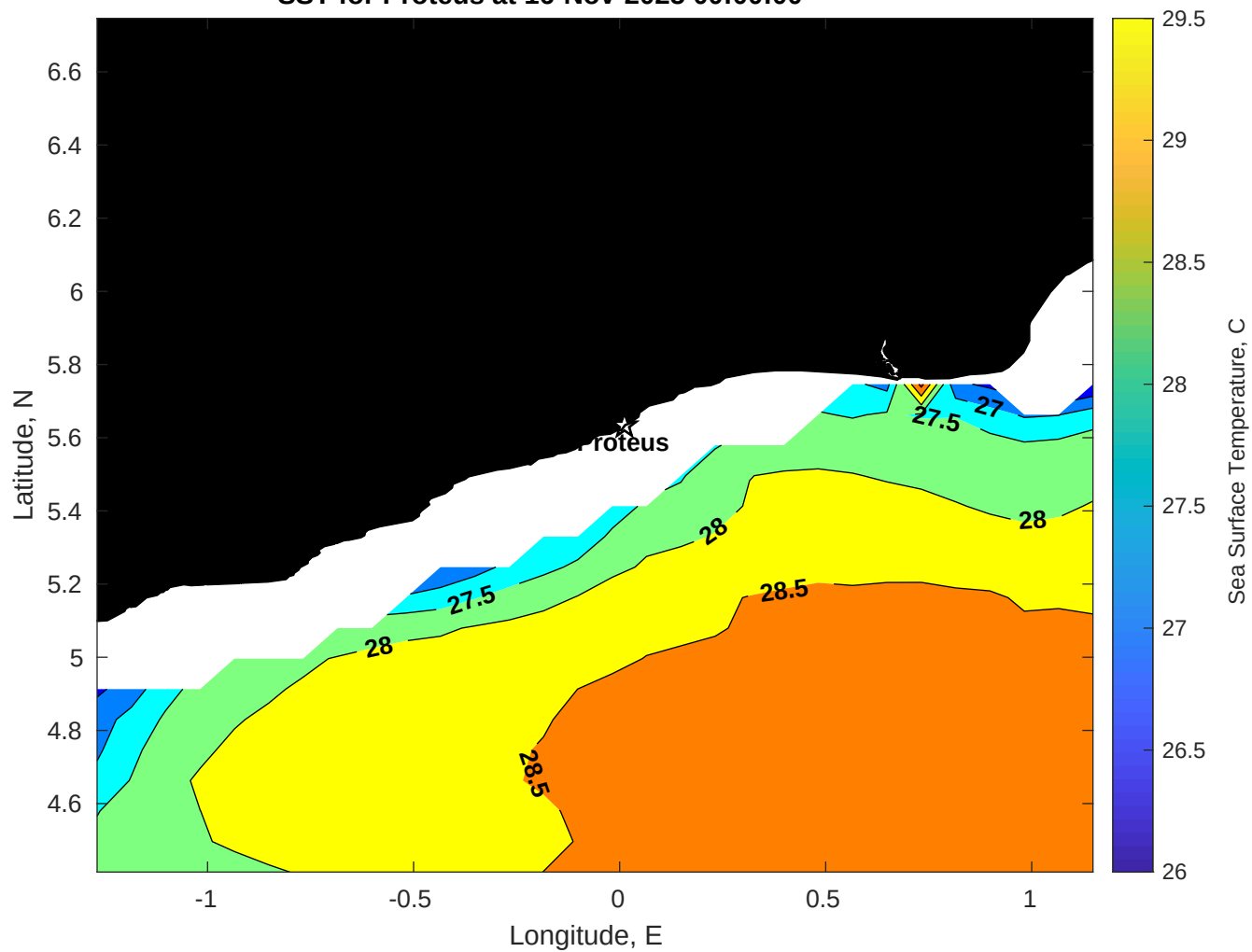
SST for Proteus at 16-Nov-2025 00:00:00
