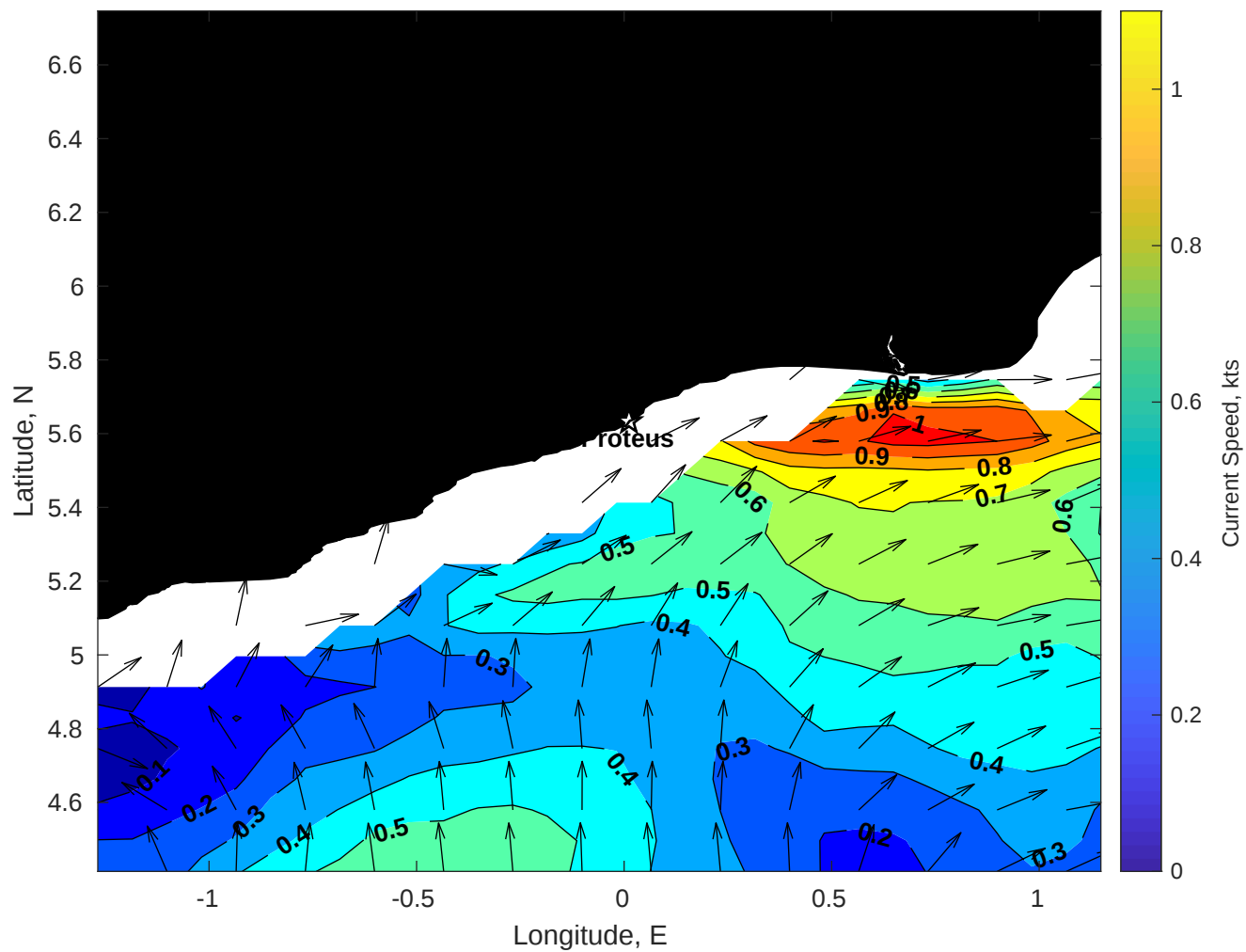
Surface Currents for Proteus at 16-Nov-2025 00:00:00
