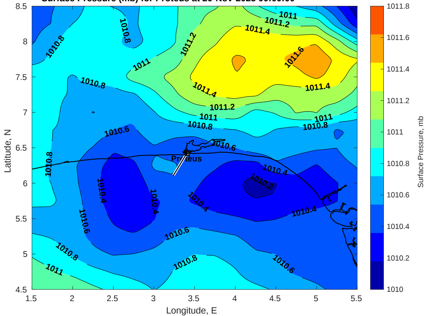
Surface Pressure (mb) for Proteus at 20-Nov-2025 00:00:00
