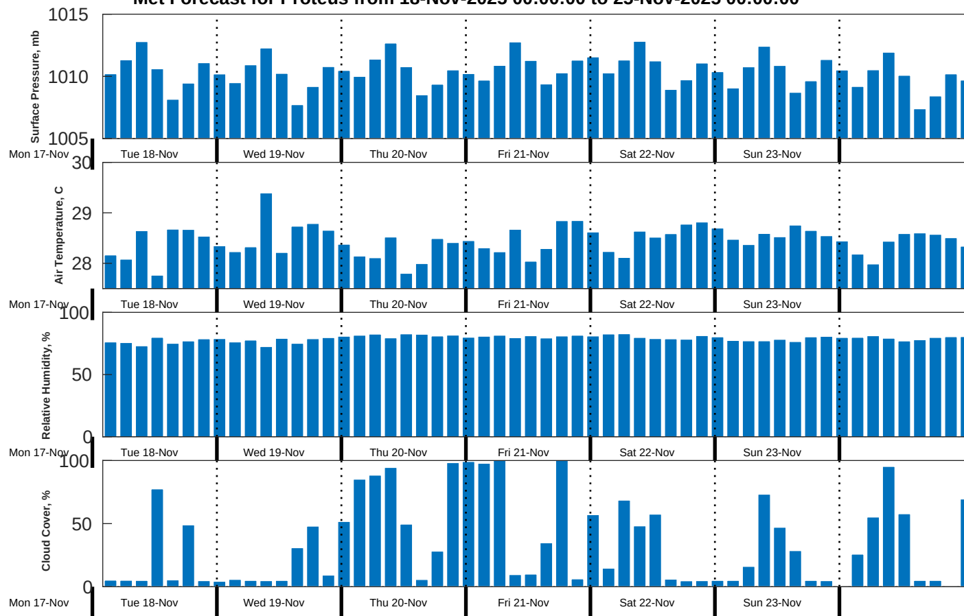
Met Forecast for Proteus from 18-Nov-2025 00:00:00 to 25-Nov-2025 00:00:00
