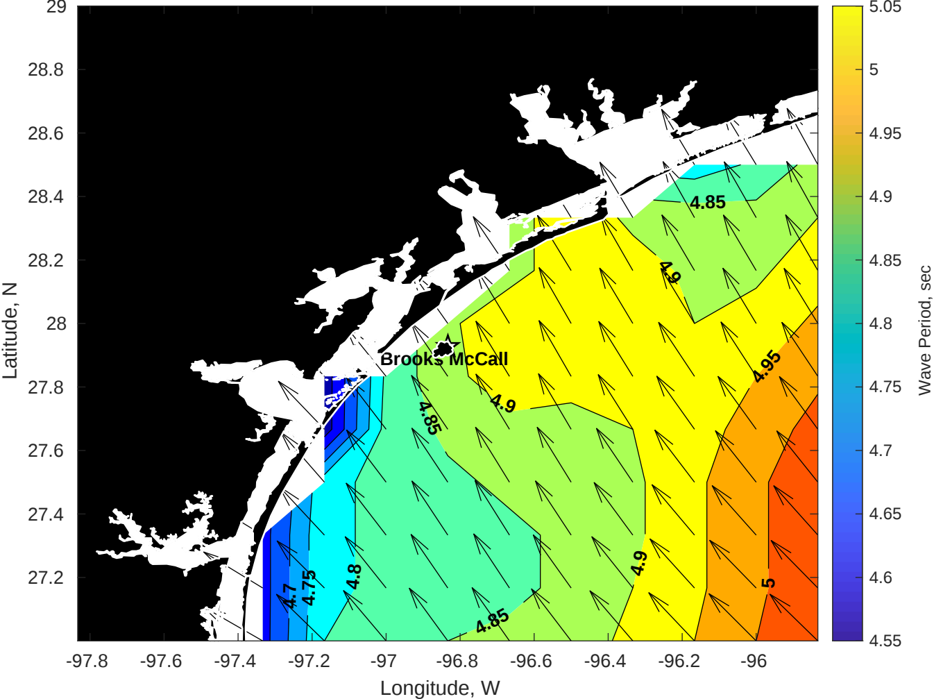
Wave Period (sec) for Brooks McCall at 19-Nov-2025 09:00:00
