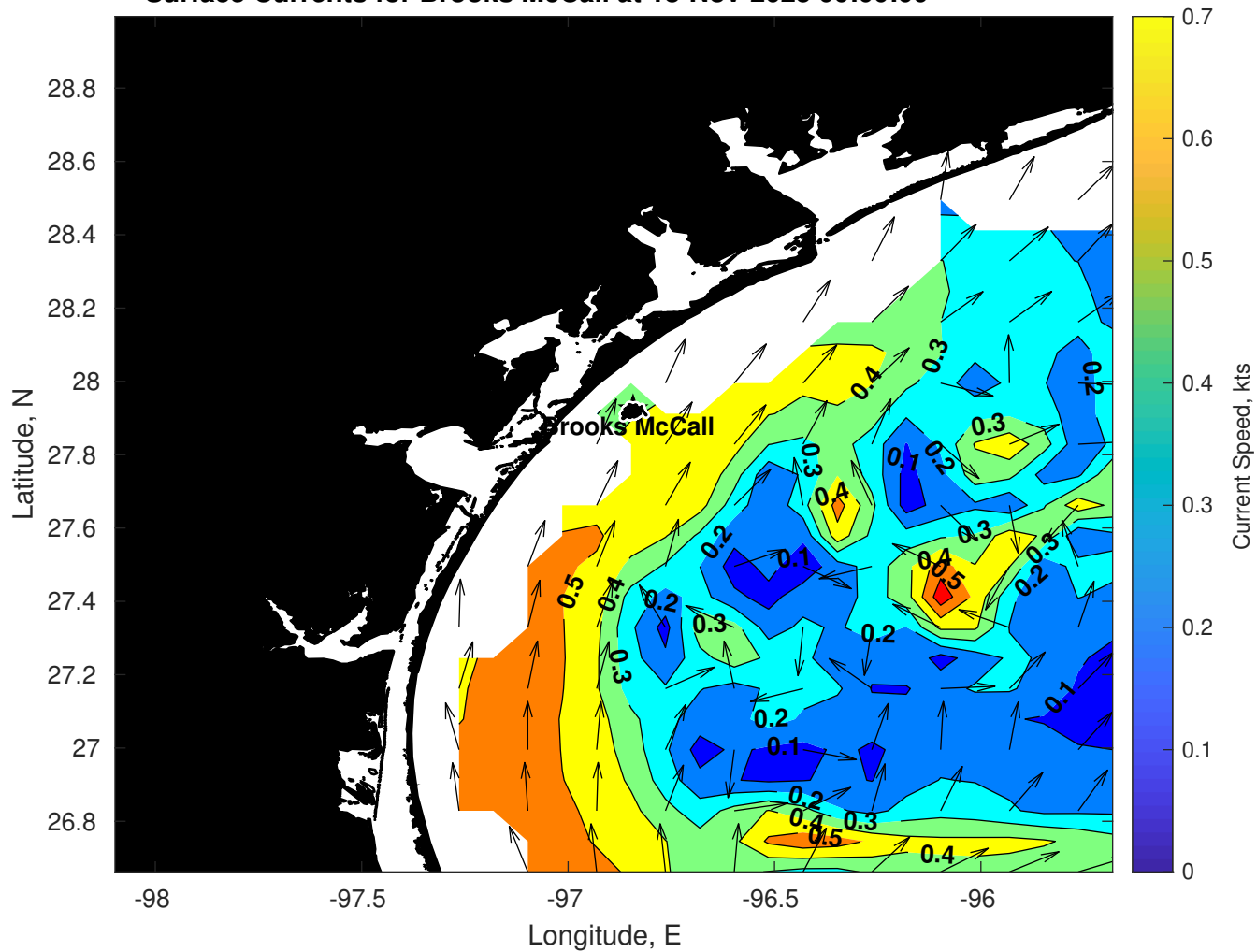
Surface Currents for Brooks McCall at 18-Nov-2025 00:00:00
