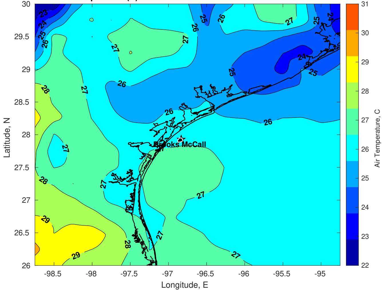
Air Temperature (C) for Brooks McCall at 19-Nov-2025
