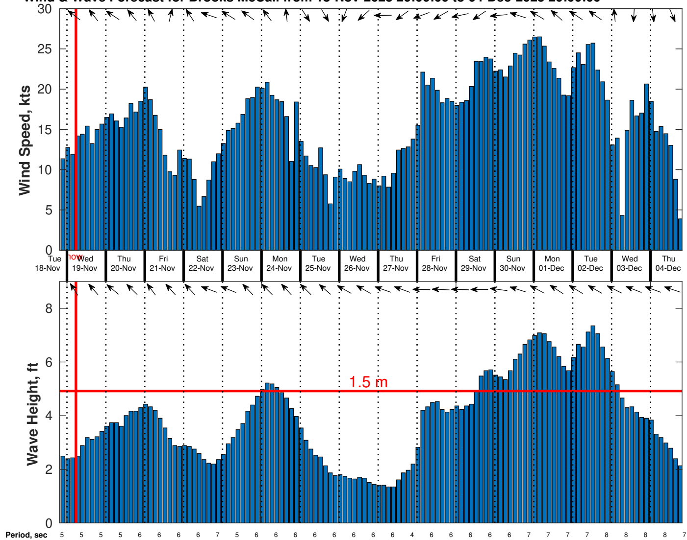
Wind & Wave Forecast for Brooks McCall from 18-Nov-2025 20:00:00 to 04-Dec-2025 20:00:00
