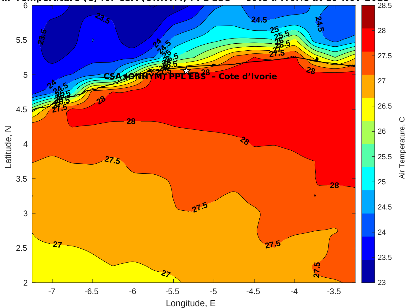
Air Temperature (C) for CSA (ONHYM) PPL EBS - Cote d'Ivoire at 19-Nov-2025
