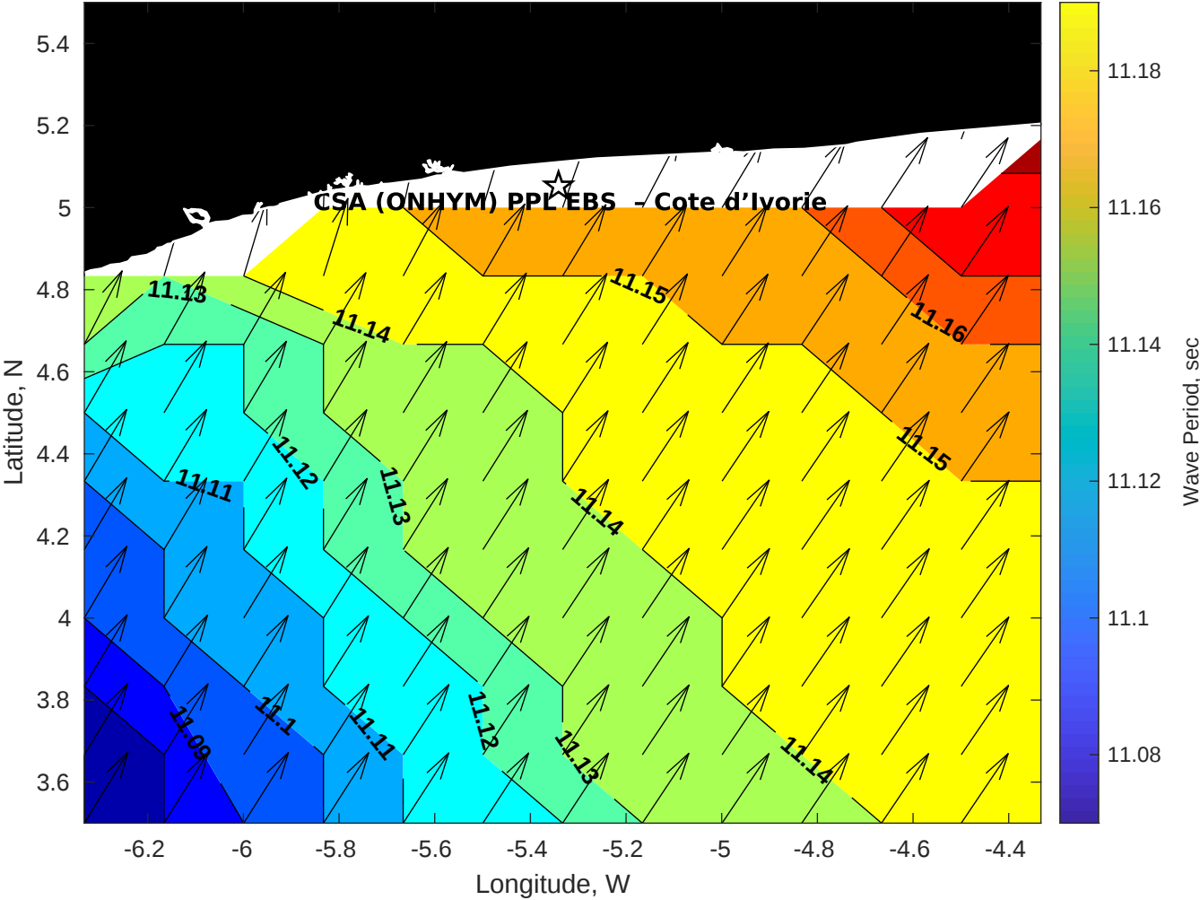
Wave Period (sec) for CSA (ONHYM) PPL EBS - Cote d'Ivoire at 19-Nov-2025 09:00:00
