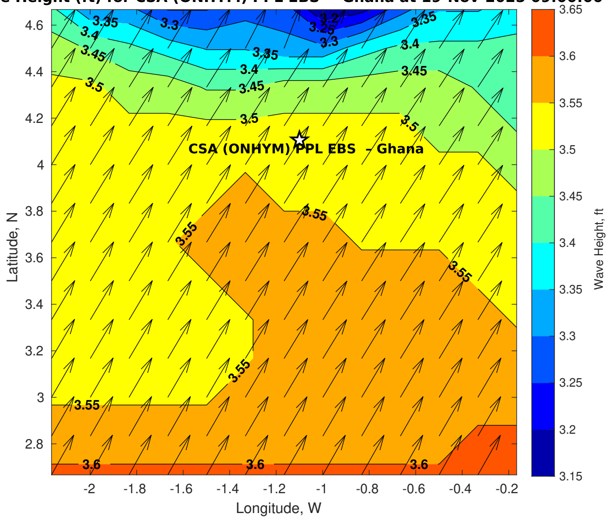
Wave Height (ft) for CSA (ONHYM) PPL EBS - Ghana at 19-Nov-2025 09:00:00
