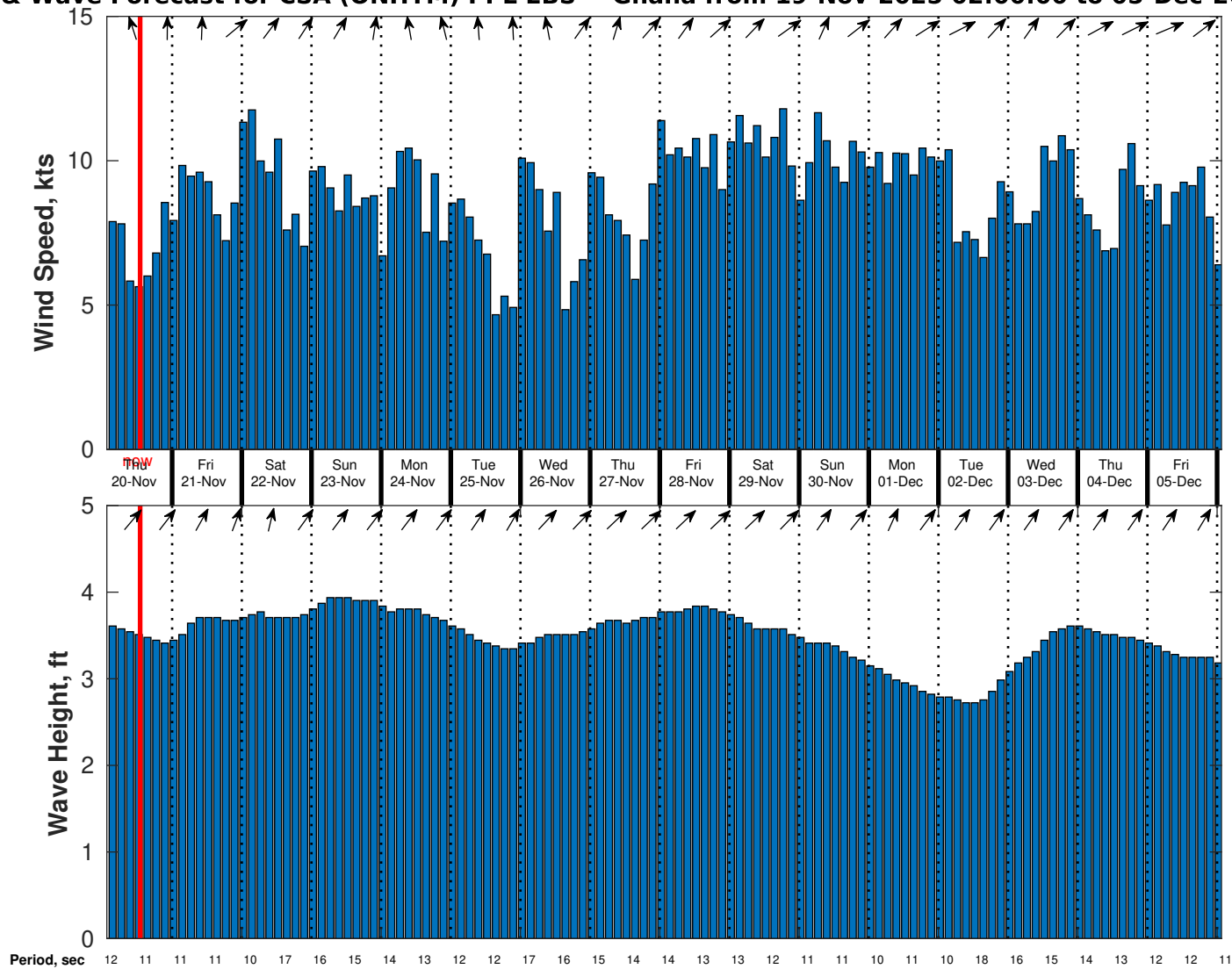
Wind & Wave Forecast for CSA (ONHYM) PPL EBS - Ghana from 19-Nov-2025 02:00:00 to 05-Dec-2025 02:00:00
