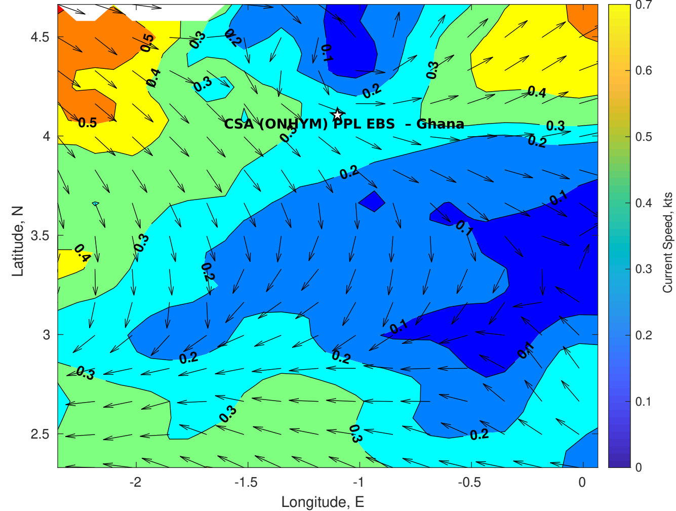
Surface Currents for CSA (ONHYM) PPL EBS - Ghana at 15-Nov-2025 00:00:00
