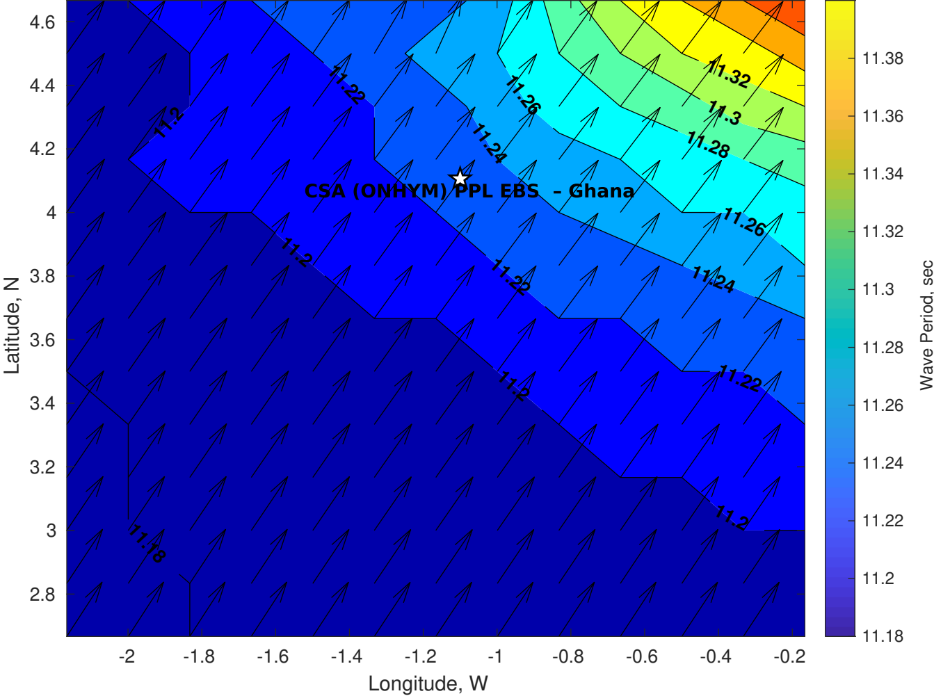
Wave Period (sec) for CSA (ONHYM) PPL EBS - Ghana at 19-Nov-2025 09:00:00
