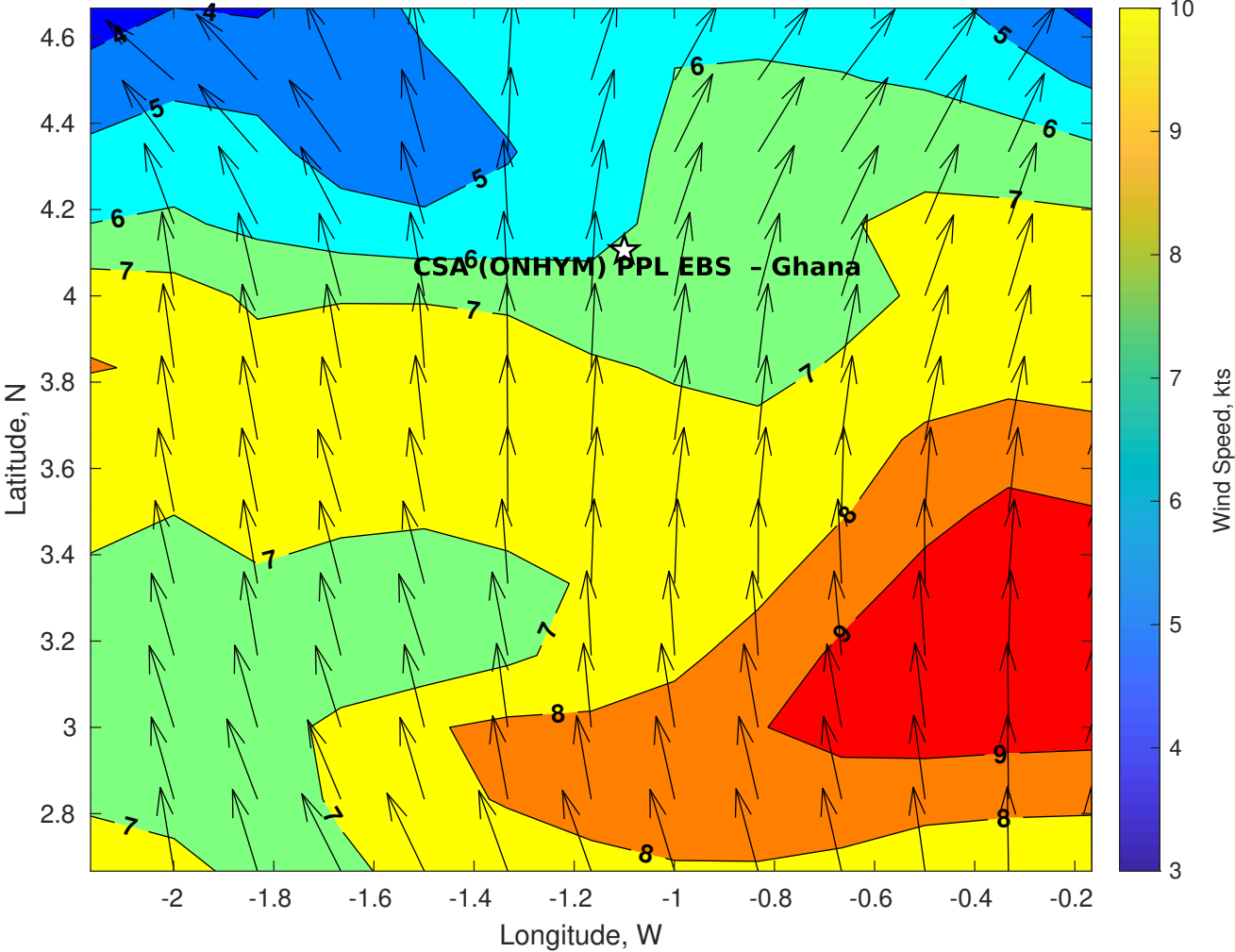
Winds (kts) for CSA (ONHYM) PPL EBS - Ghana at 19-Nov-2025 09:00:00
