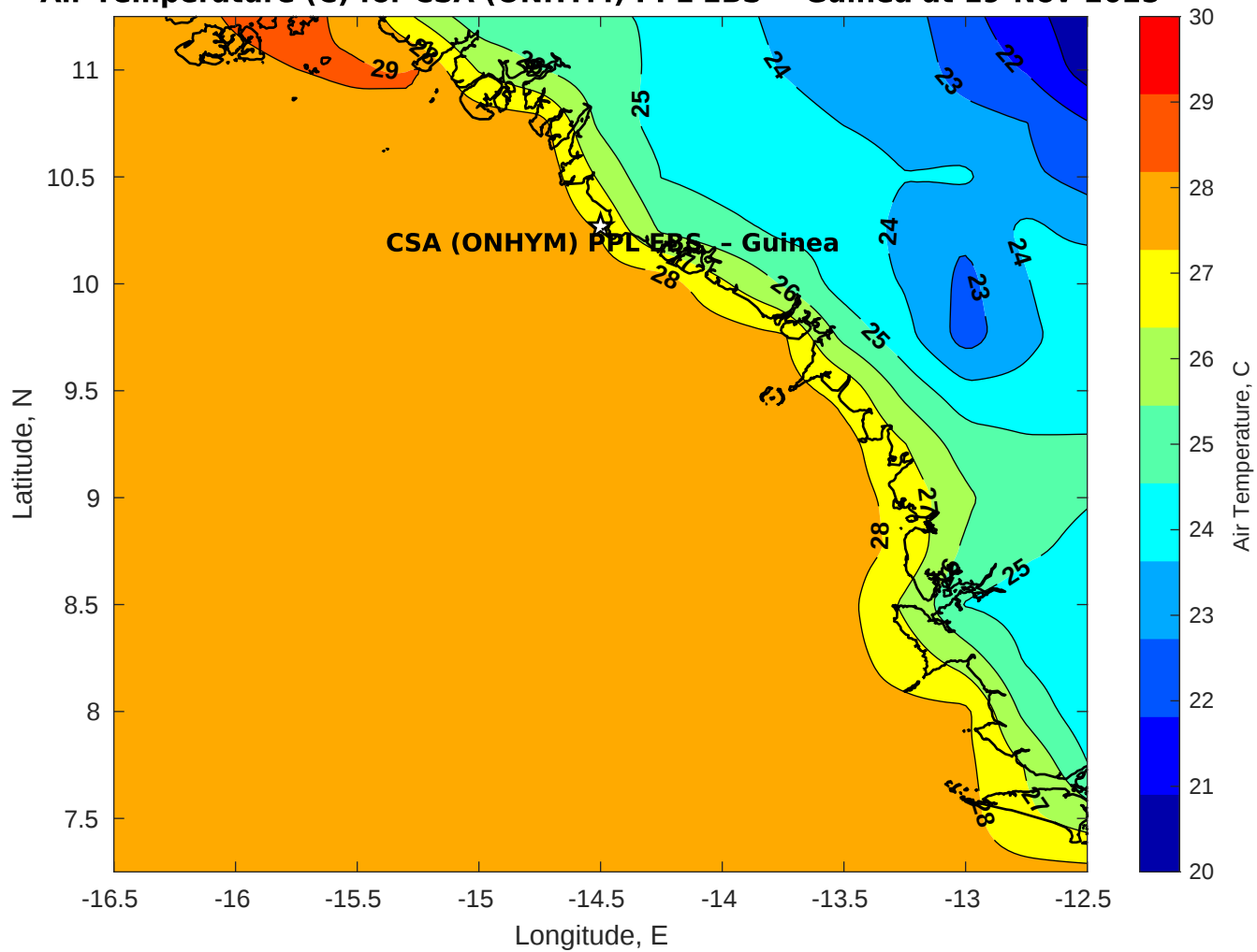
Air Temperature (C) for CSA (ONHYM) PPL EBS - Guinea at 19-Nov-2025
