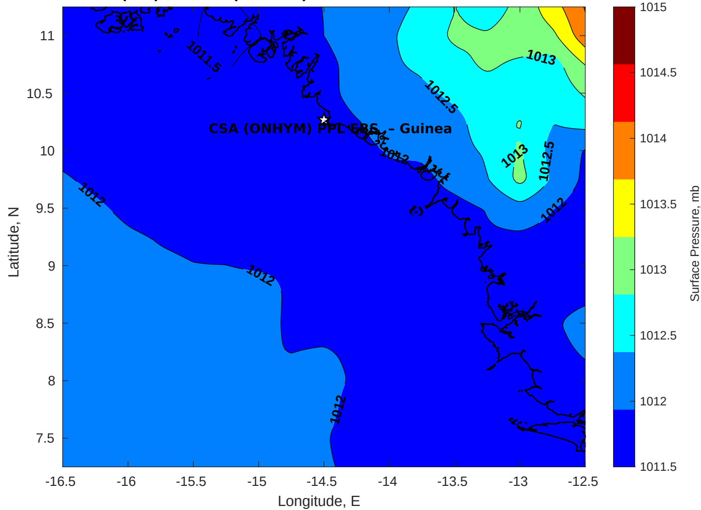
Surface Pressure (mb) for CSA (ONHYM) PPL EBS - Guinea at 19-Nov-2025 00:00:00
