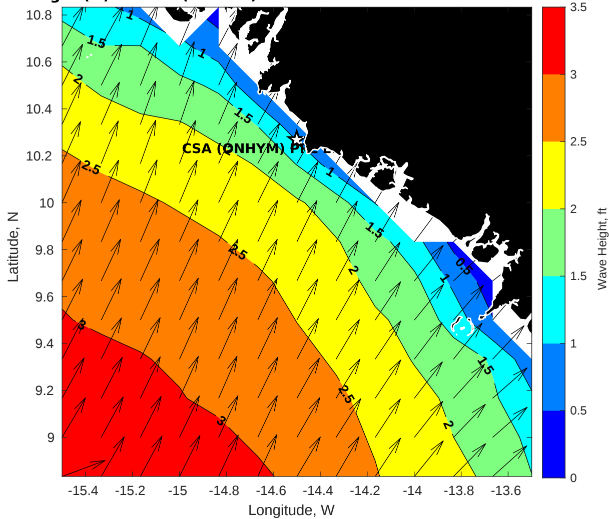
Wave Height (ft) for CSA (ONHYM) PPL EBS - Guinea at 19-Nov-2025 09:00:00
