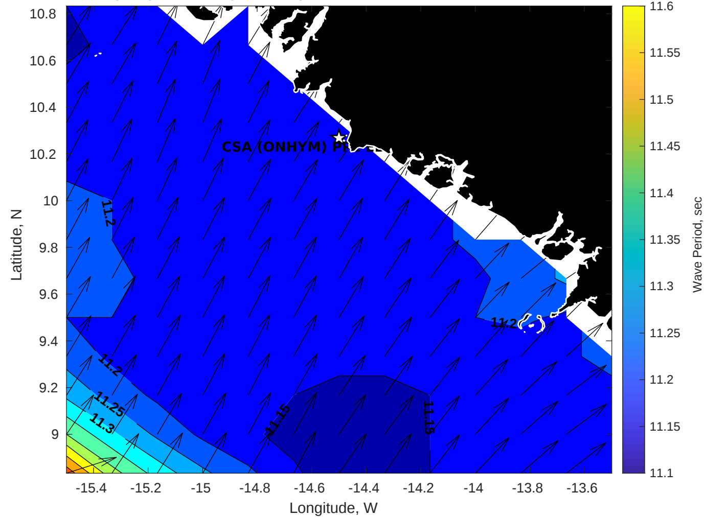
Wave Period (sec) for CSA (ONHYM) PPL EBS - Guinea at 19-Nov-2025 09:00:00
