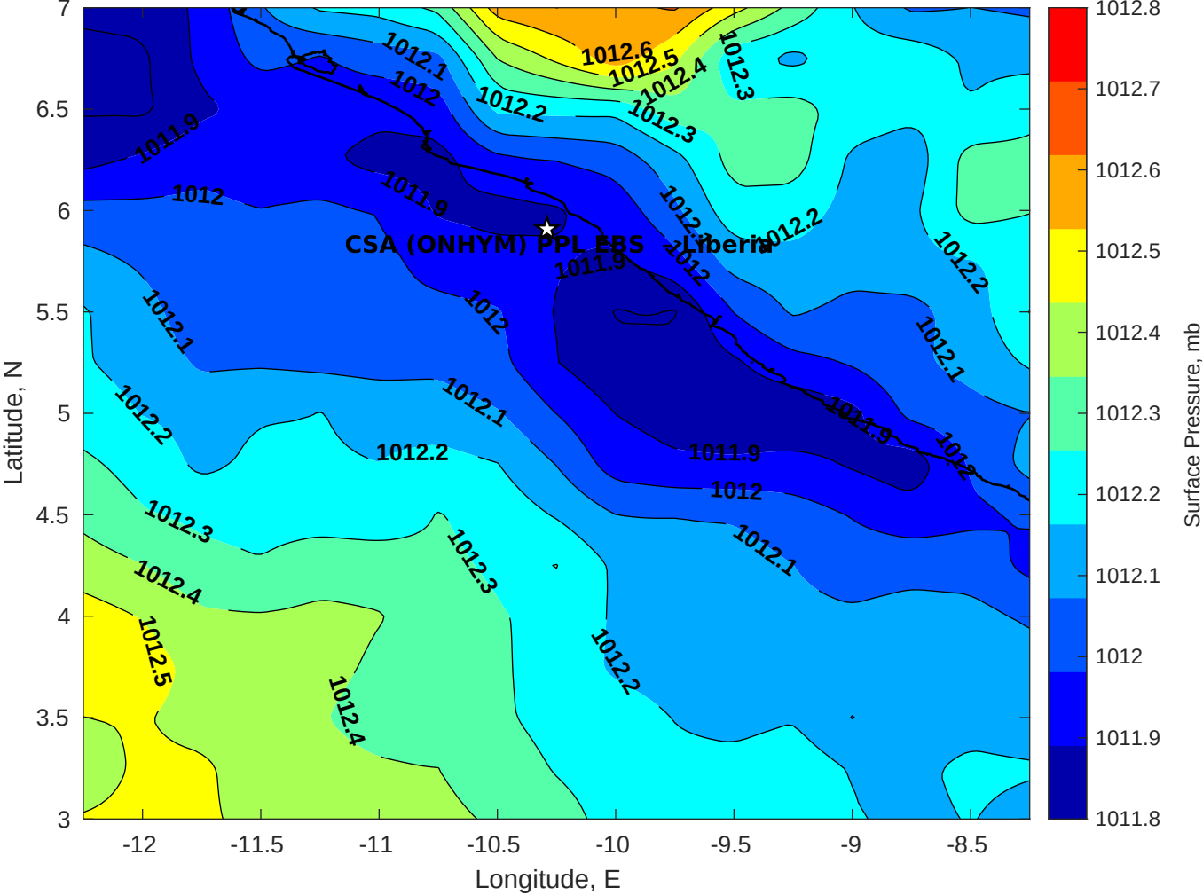
Surface Pressure (mb) for CSA (ONHYM) PPL EBS - Liberia at 20-Nov-2025 00:00:00
