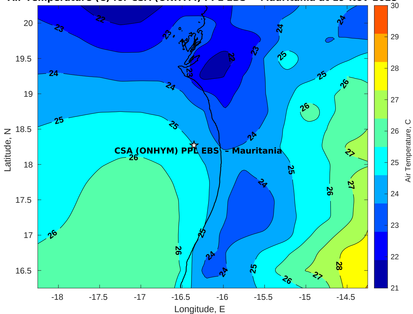
Air Temperature (C) for CSA (ONHYM) PPL EBS - Mauritania at 19-Nov-2025
