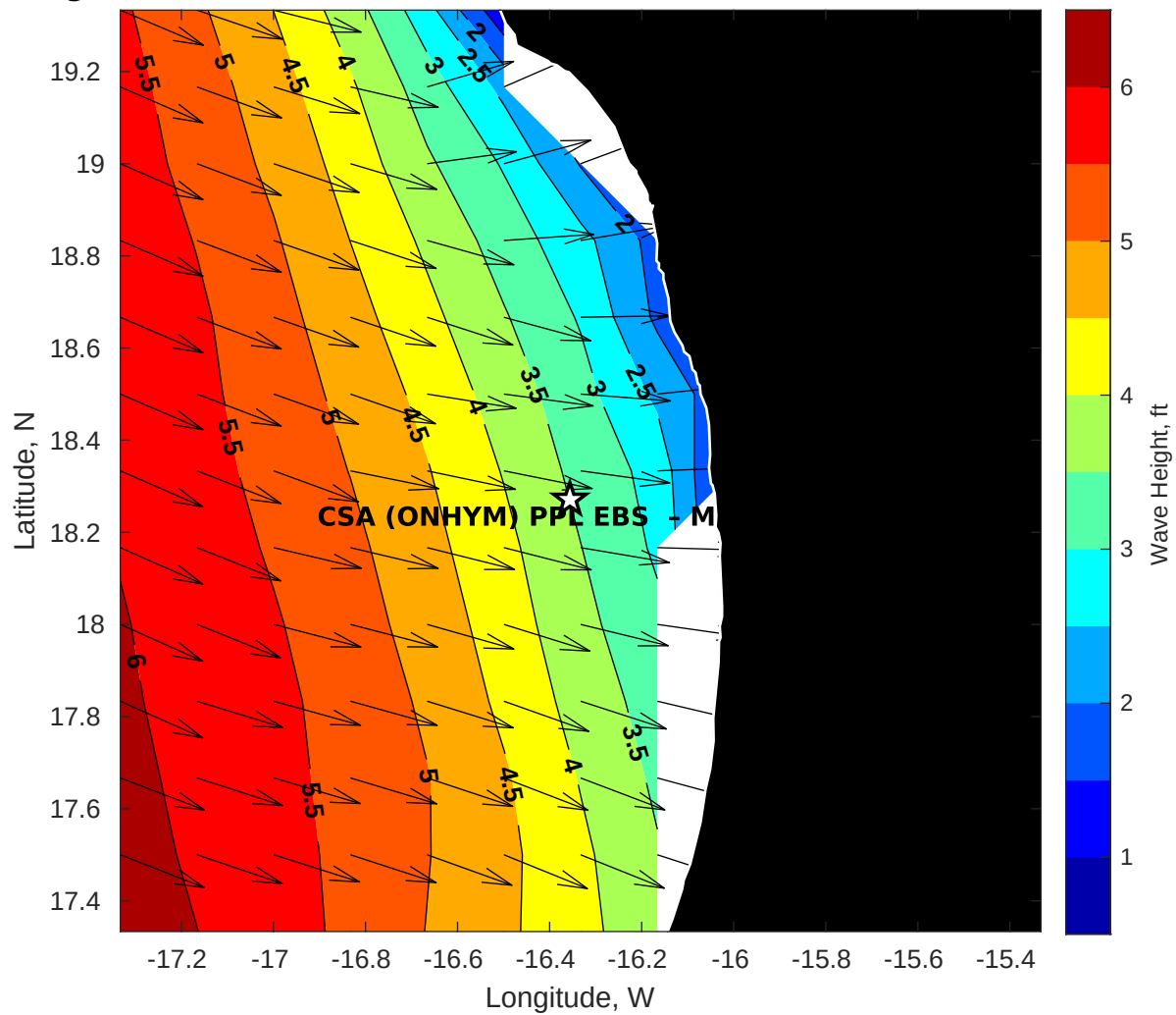
Wave Height (ft) for CSA (ONHYM) PPL EBS - Mauritania at 19-Nov-2025 09:00:00
