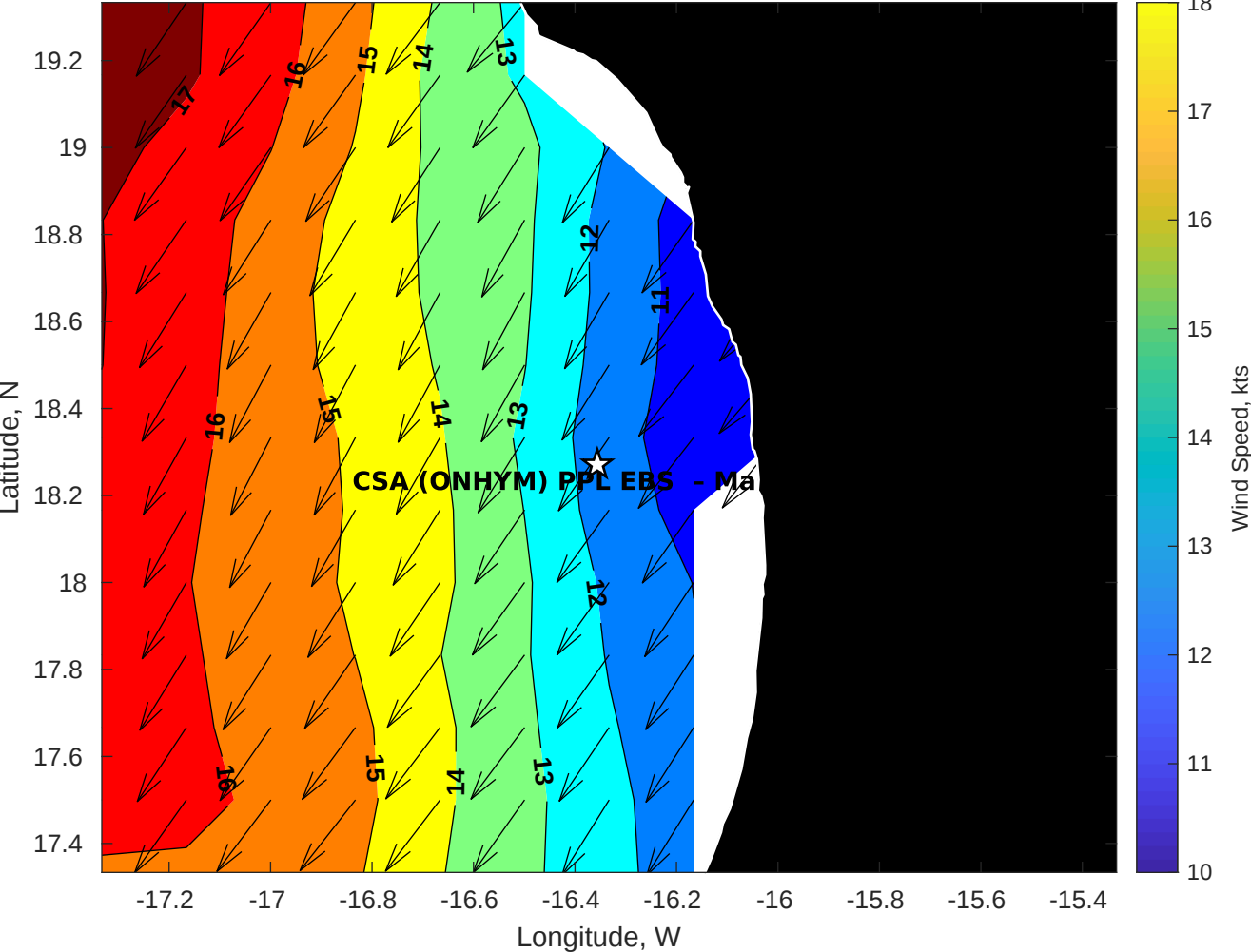
Winds (kts) for CSA (ONHYM) PPL EBS - Mauritania at 19-Nov-2025 09:00:00
