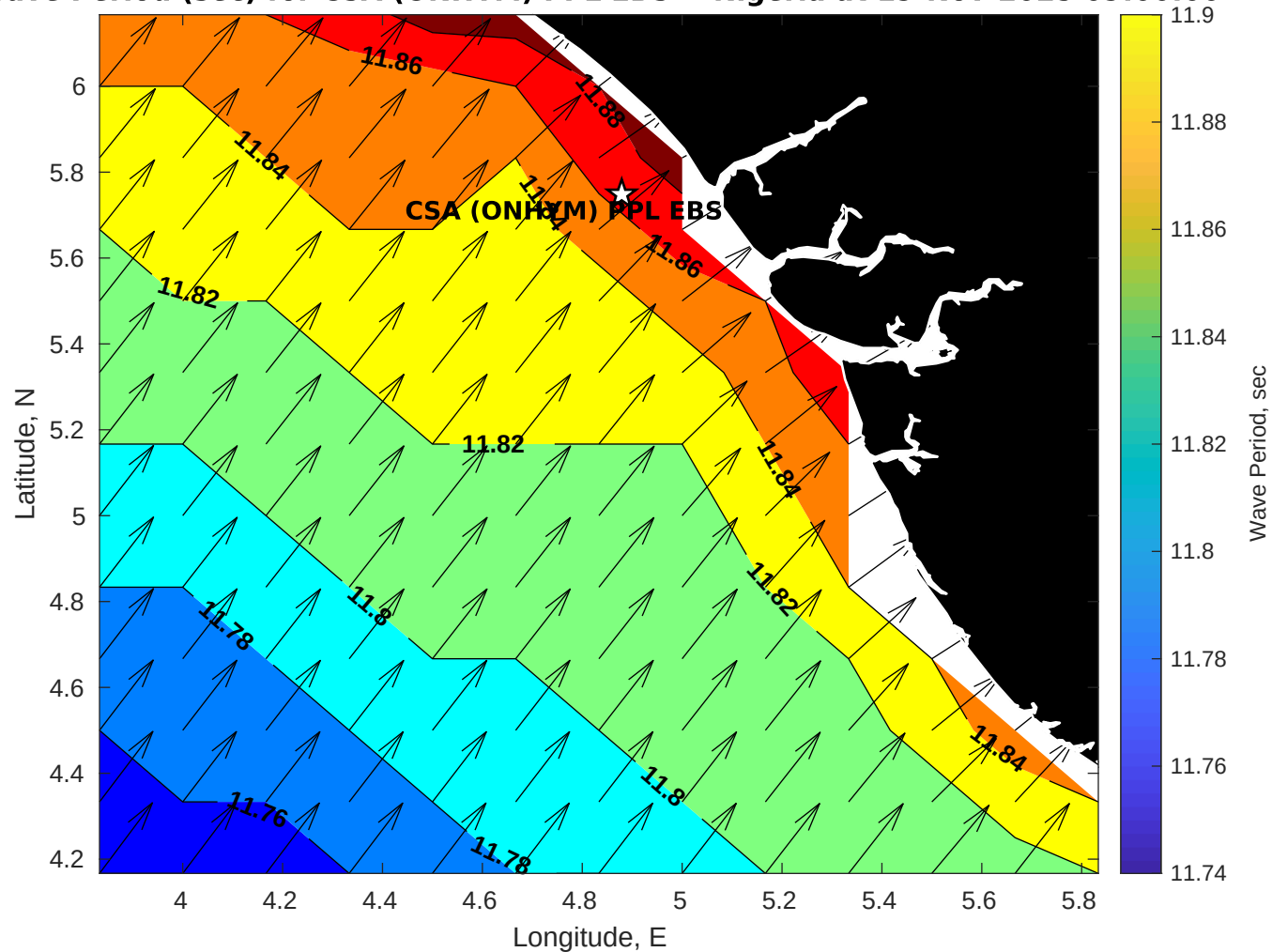
Wave Period (sec) for CSA (ONHYM) PPL EBS - Nigeria at 19-Nov-2025 09:00:00
