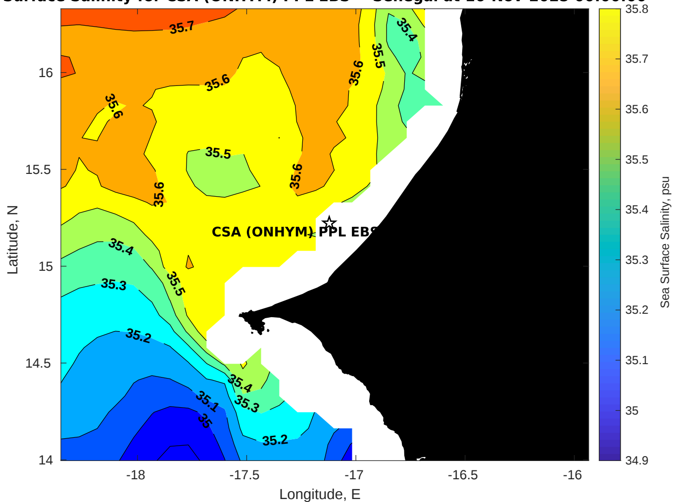
Surface Salinity for CSA (ONHYM) PPL EBS - Senegal at 16-Nov-2025 00:00:00
