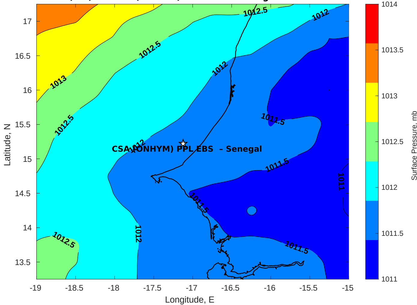
Surface Pressure (mb) for CSA (ONHYM) PPL EBS - Senegal at 20-Nov-2025 00:00:00
