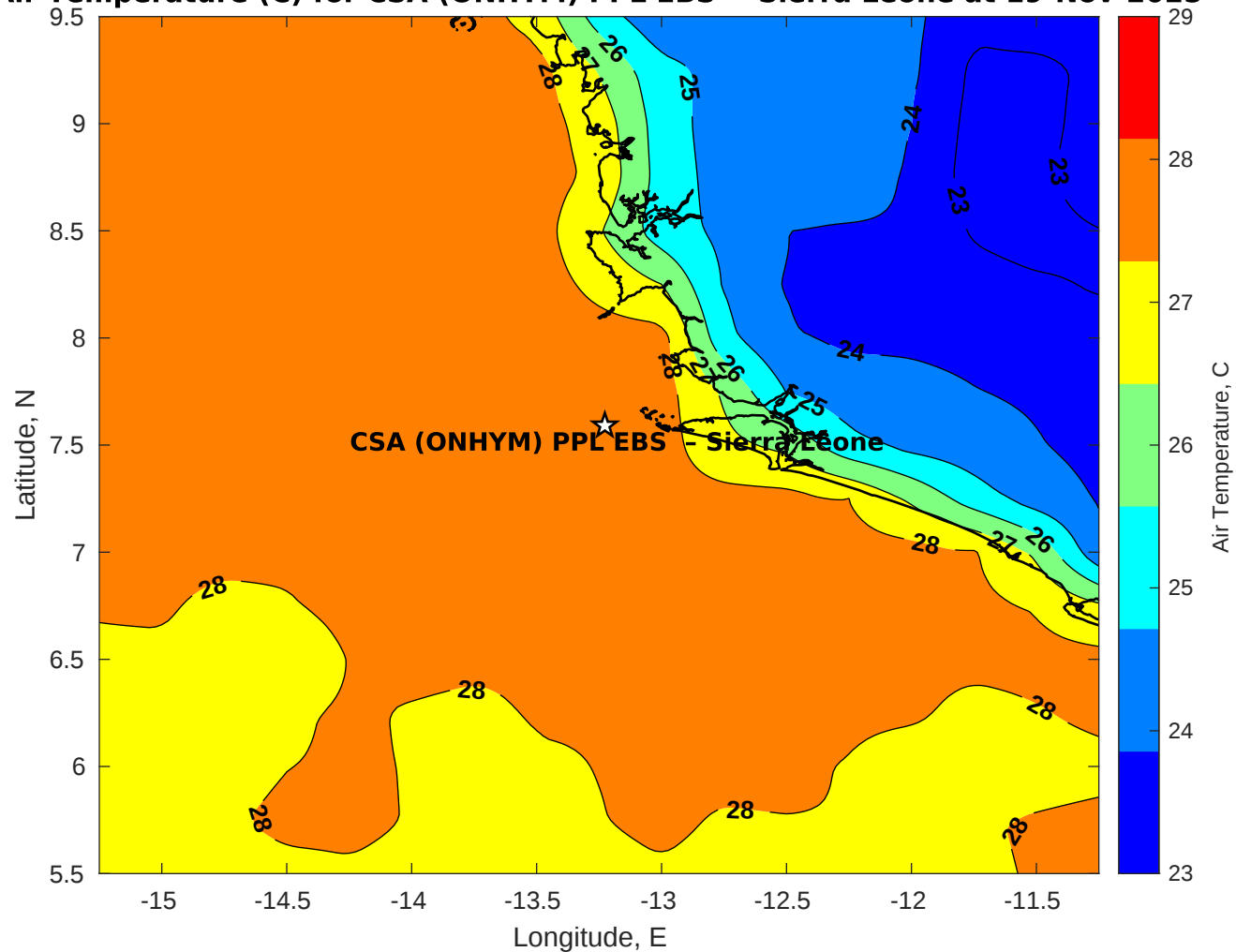
Air Temperature (C) for CSA (ONHYM) PPL EBS - Sierra Leone at 19-Nov-2025
