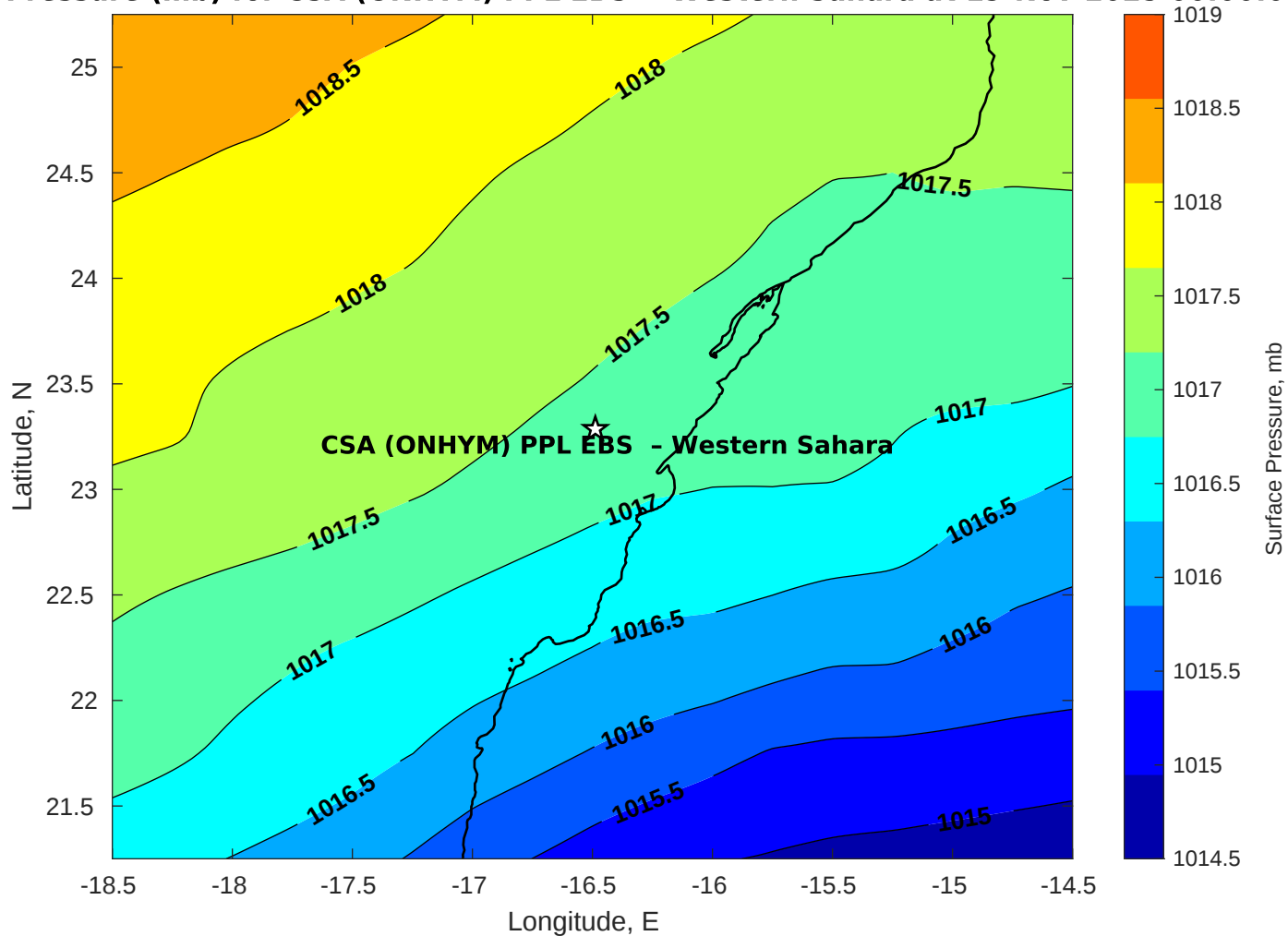
Surface Pressure (mb) for CSA (ONHYM) PPL EBS - Western Sahara at 19-Nov-2025 00:00:00
