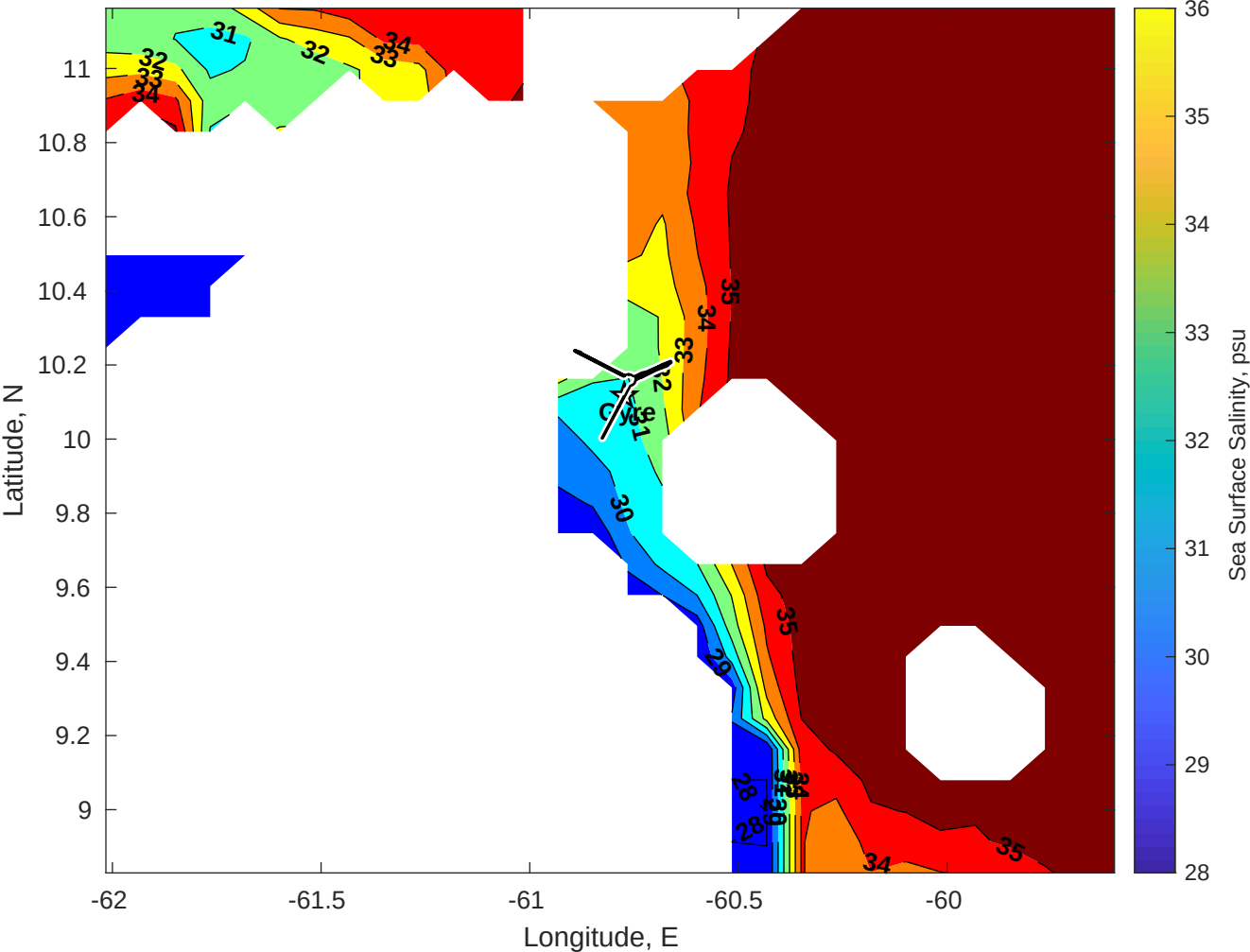
Surface Salinity for Gyre at 18-Nov-2025 00:00:00
