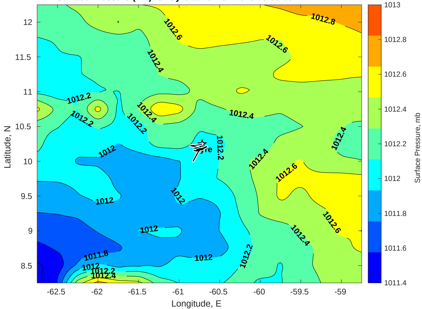
Surface Pressure (mb) for Gyre at 20-Nov-2025 00:00:00
