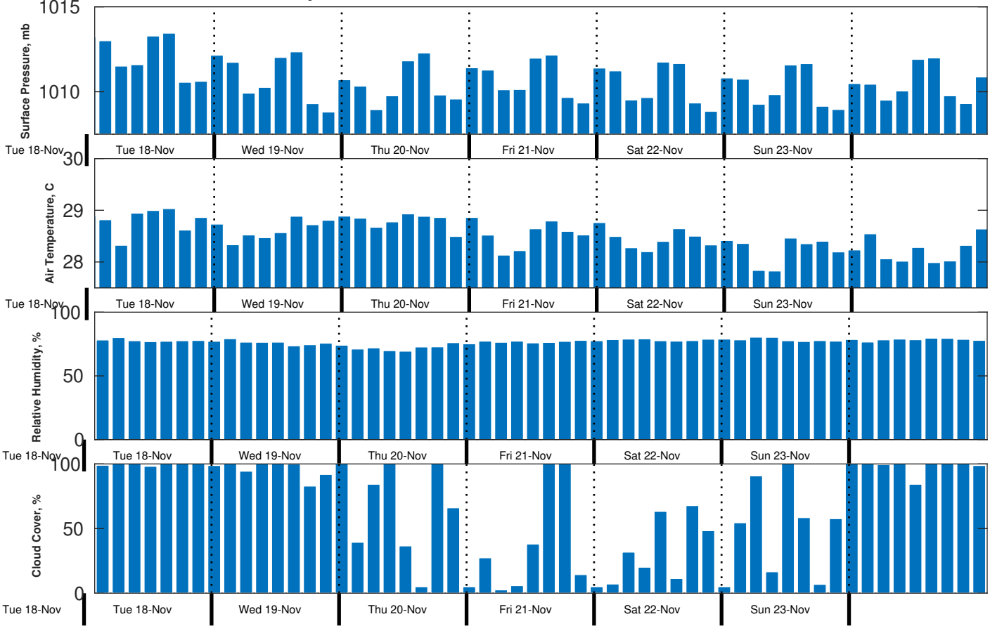
Met Forecast for Gyre from 18-Nov-2025 20:00:00 to 25-Nov-2025 20:00:00
