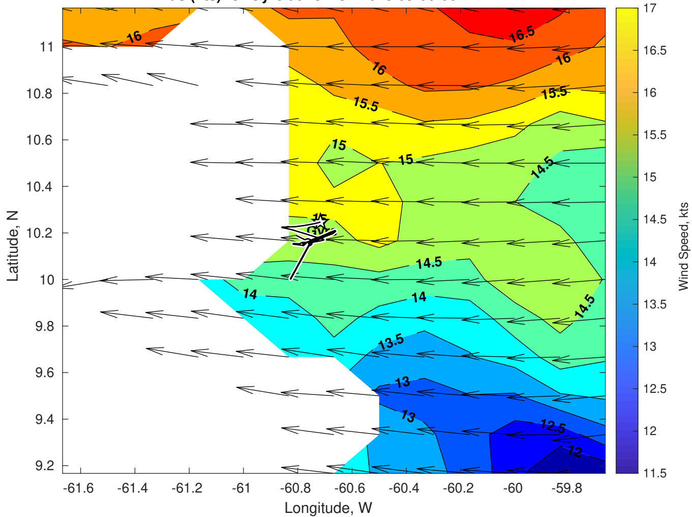
Winds (kts) for Gyre at 19-Nov-2025 09:00:00
