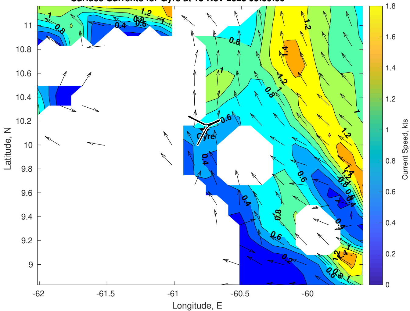
Surface Currents for Gyre at 18-Nov-2025 00:00:00
