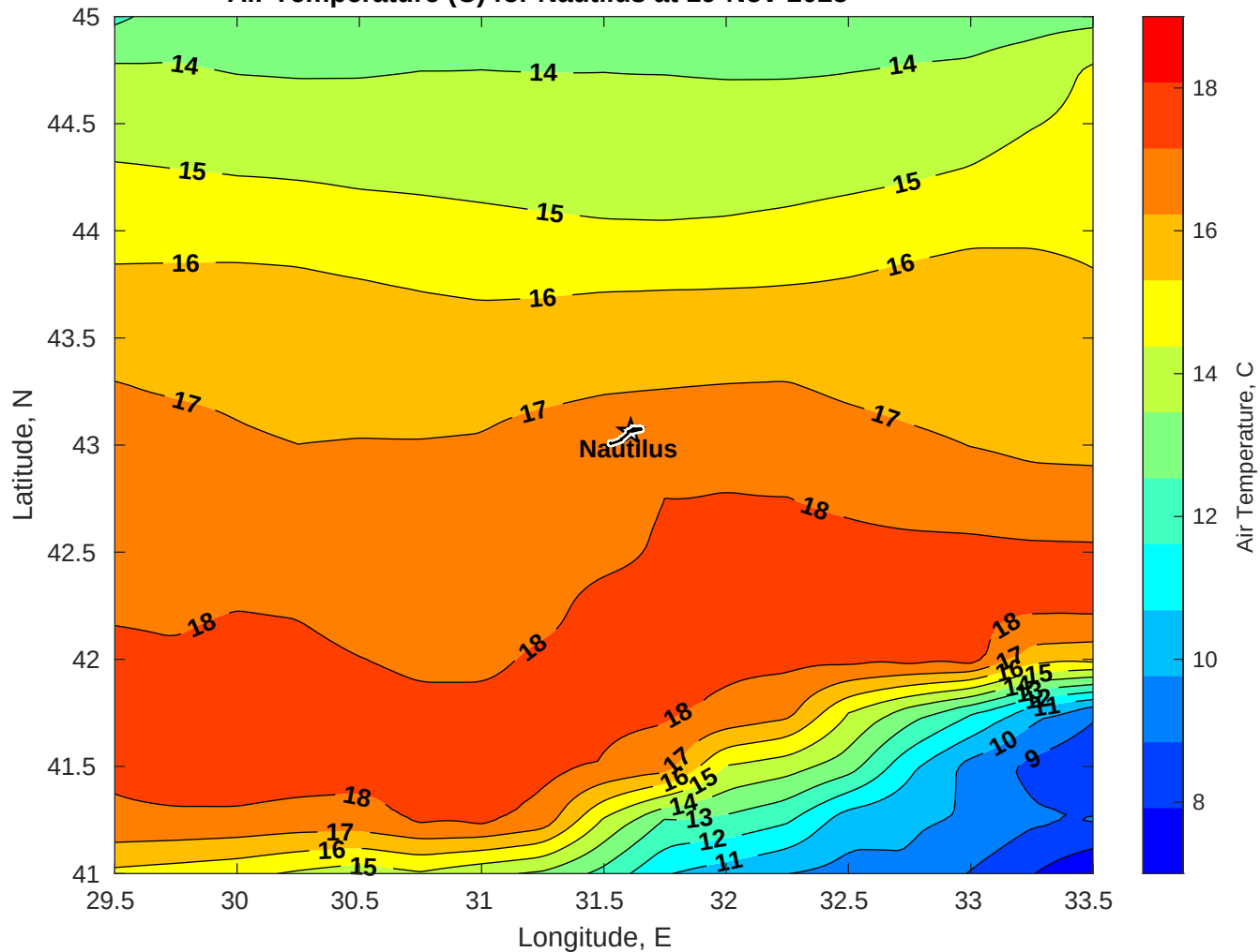
Air Temperature (C) for Nautilus at 19-Nov-2025
