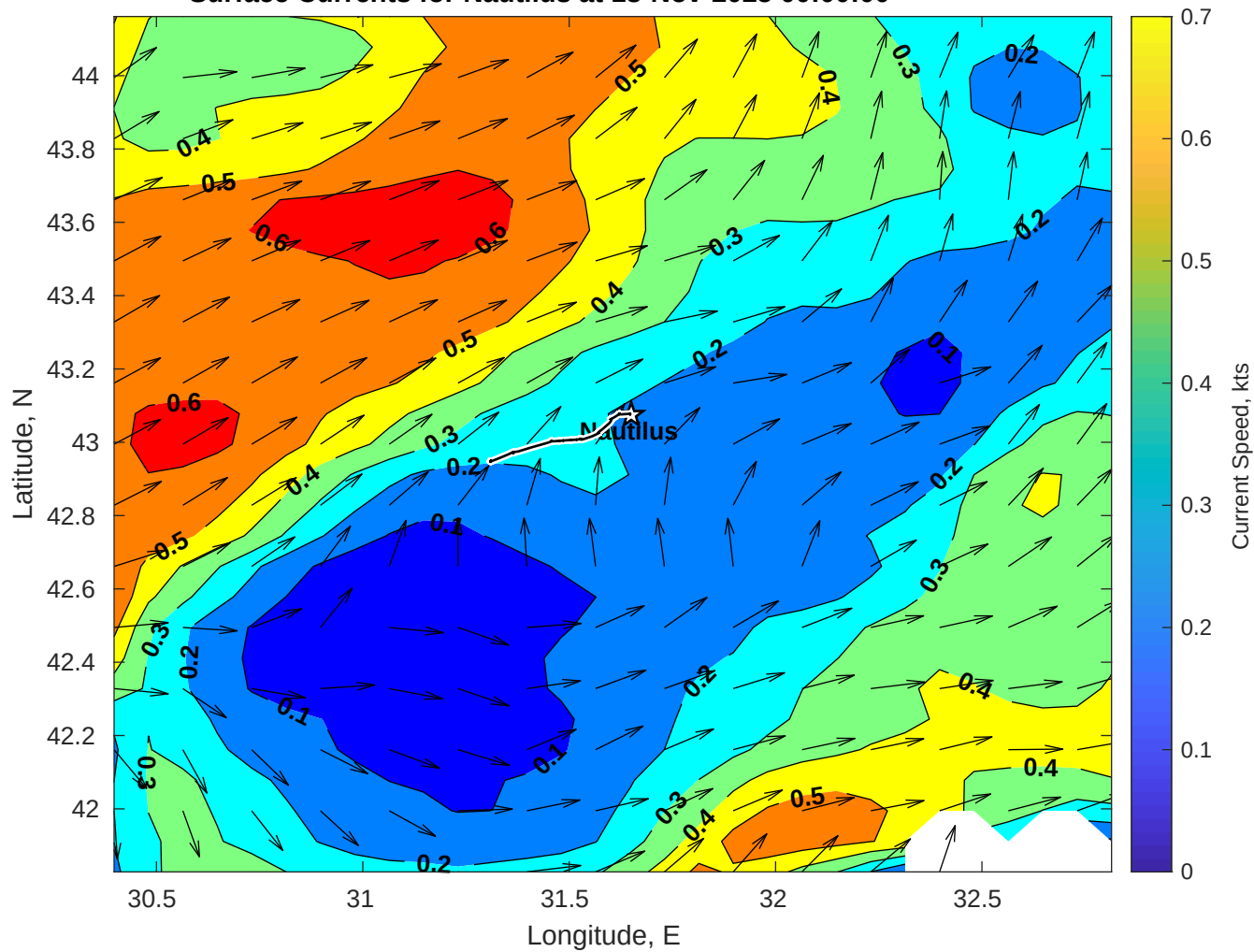
Surface Currents for Nautilus at 18-Nov-2025 00:00:00
