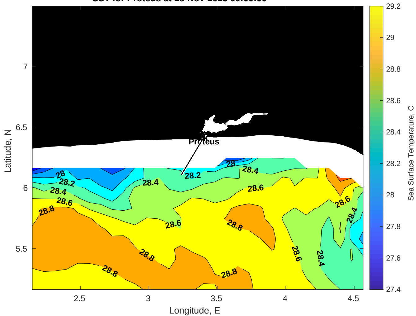
SST for Proteus at 18-Nov-2025 00:00:00
