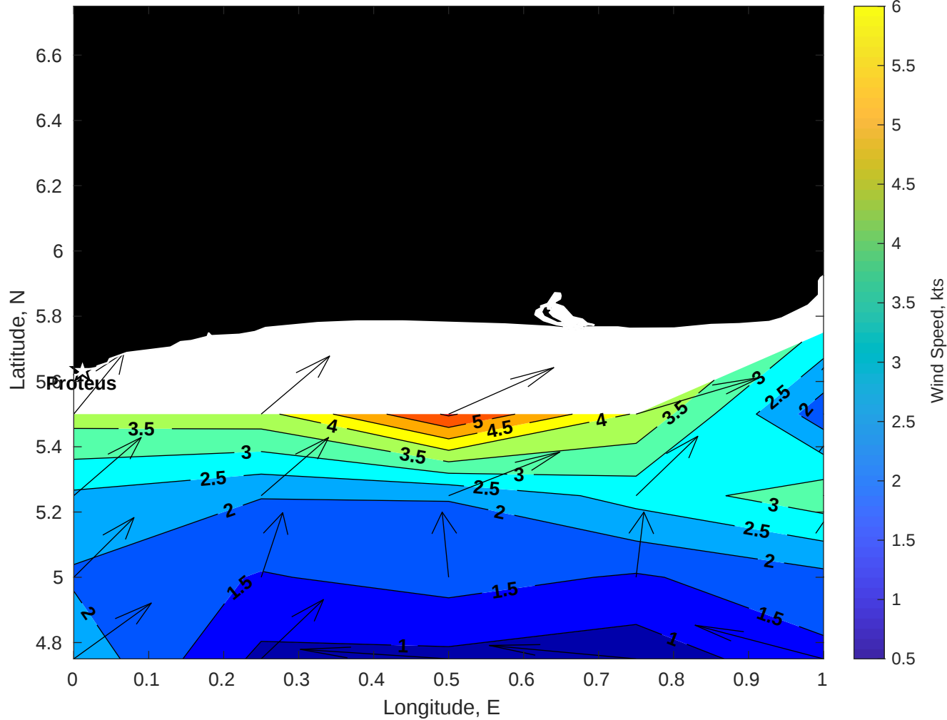
Winds (kts) for Proteus at 19-Nov-2025 09:00:00
