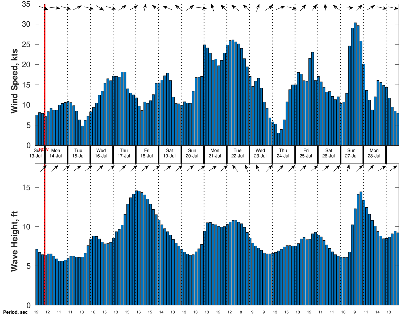
Wind & Wave Forecast for Benthic Solutions South Africa HF Site2 from 13-Jul-2025 14:00:00 to 29-Jul-2025 14:00:00
