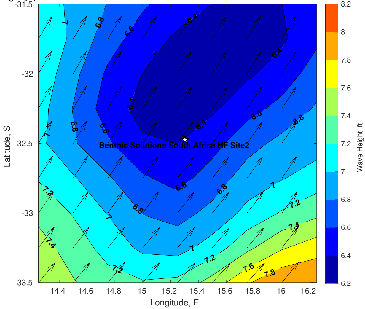
Wave Height (ft) for Benthic Solutions South Africa HF Site2 at 13-Jul-2025 21:00:00
