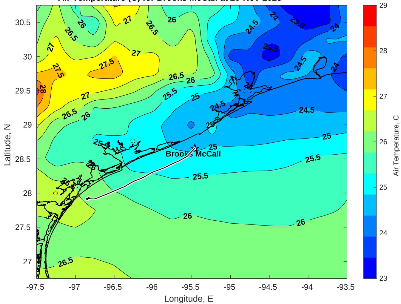
Air Temperature (C) for Brooks McCall at 20-Nov-2025
