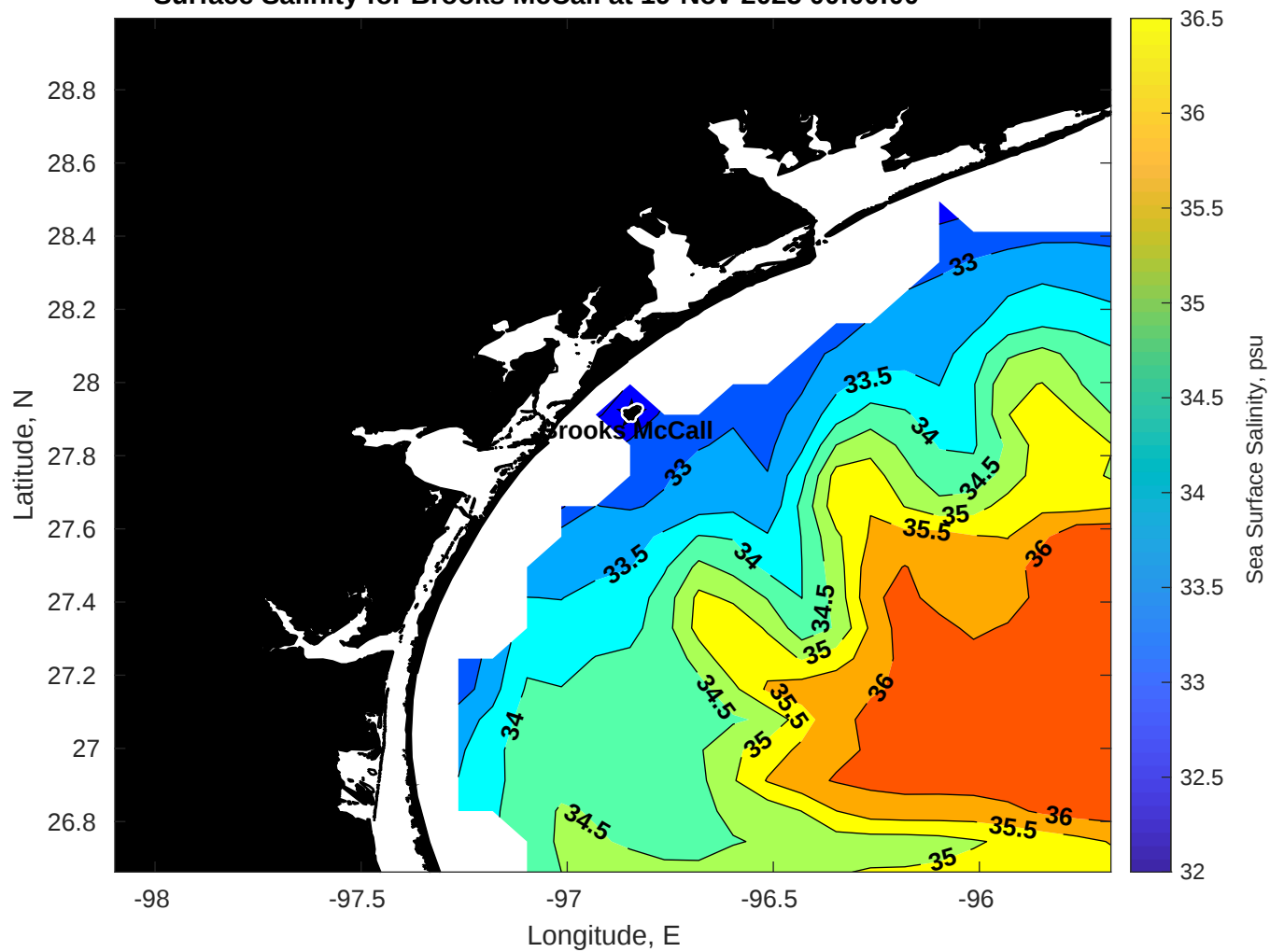
Surface Salinity for Brooks McCall at 19-Nov-2025 00:00:00
