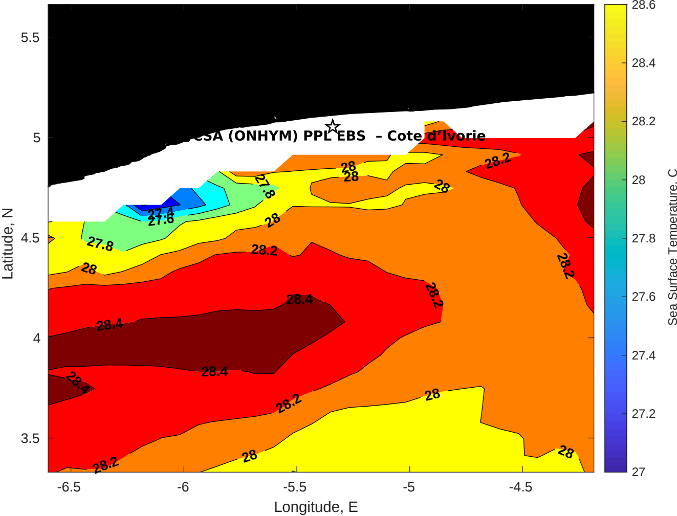
SST for CSA (ONHYM) PPL EBS - Cote d'Ivoire at 19-Nov-2025 00:00:00
