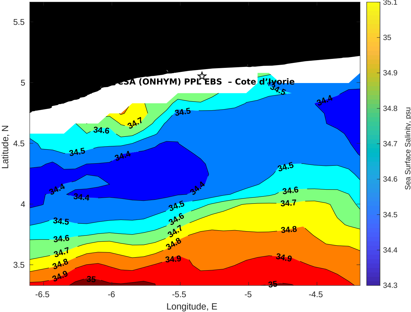
Surface Salinity for CSA (ONHYM) PPL EBS - Cote d'Ivoire at 19-Nov-2025 00:00:00
