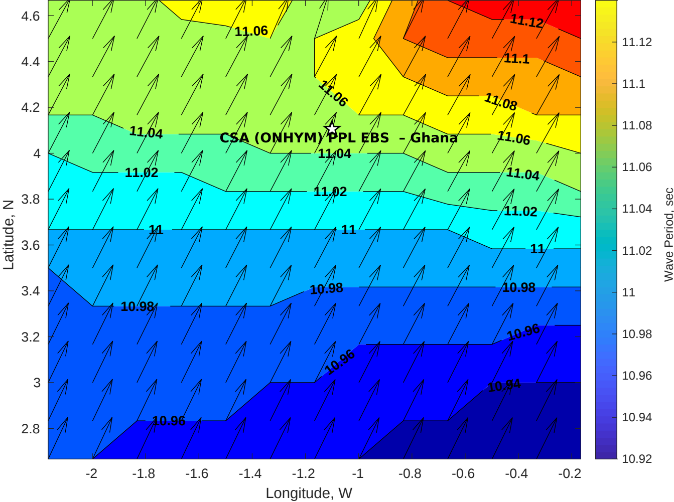
Wave Period (sec) for CSA (ONHYM) PPL EBS - Ghana at 19-Nov-2025 21:00:00
