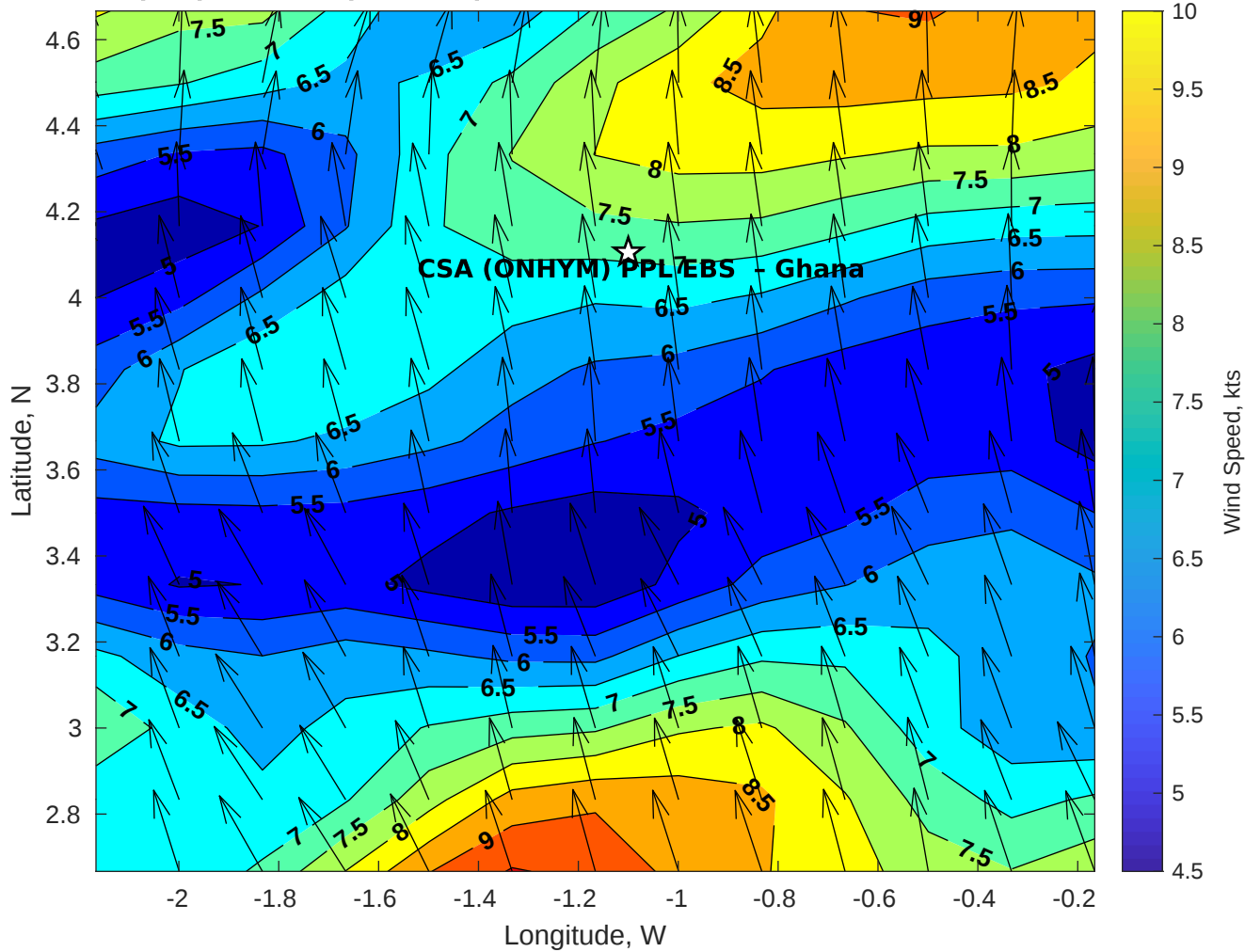
Winds (kts) for CSA (ONHYM) PPL EBS - Ghana at 19-Nov-2025 21:00:00
