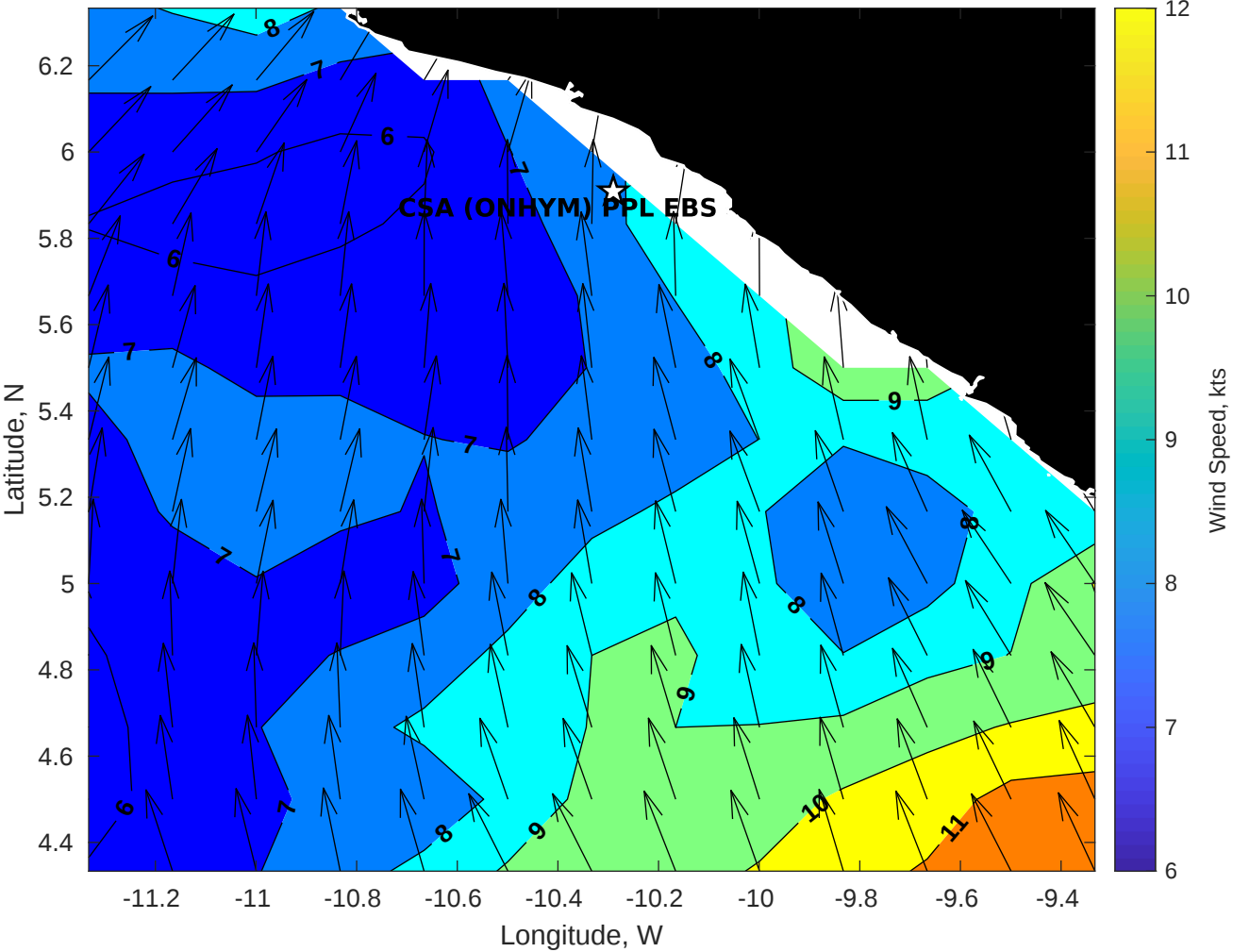
Winds (kts) for CSA (ONHYM) PPL EBS - Liberia at 19-Nov-2025 21:00:00
