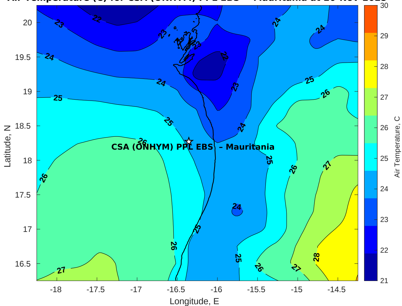
Air Temperature (C) for CSA (ONHYM) PPL EBS - Mauritania at 20-Nov-2025
