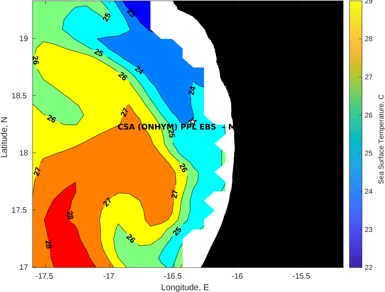
SST for CSA (ONHYM) PPL EBS - Mauritania at 19-Nov-2025 00:00:00
