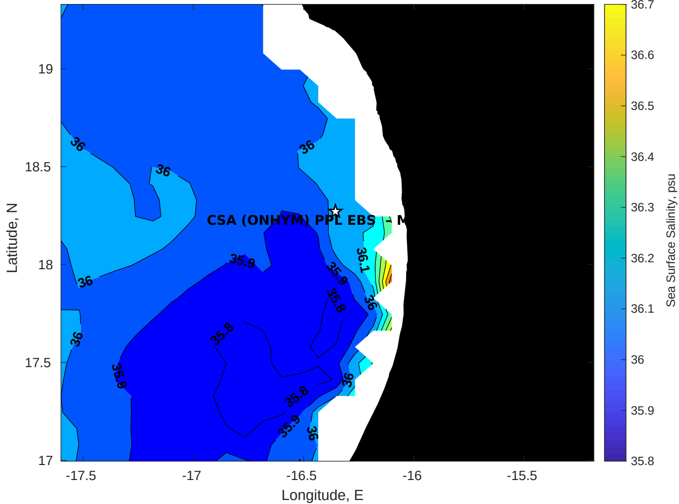
Surface Salinity for CSA (ONHYM) PPL EBS - Mauritania at 19-Nov-2025 00:00:00
