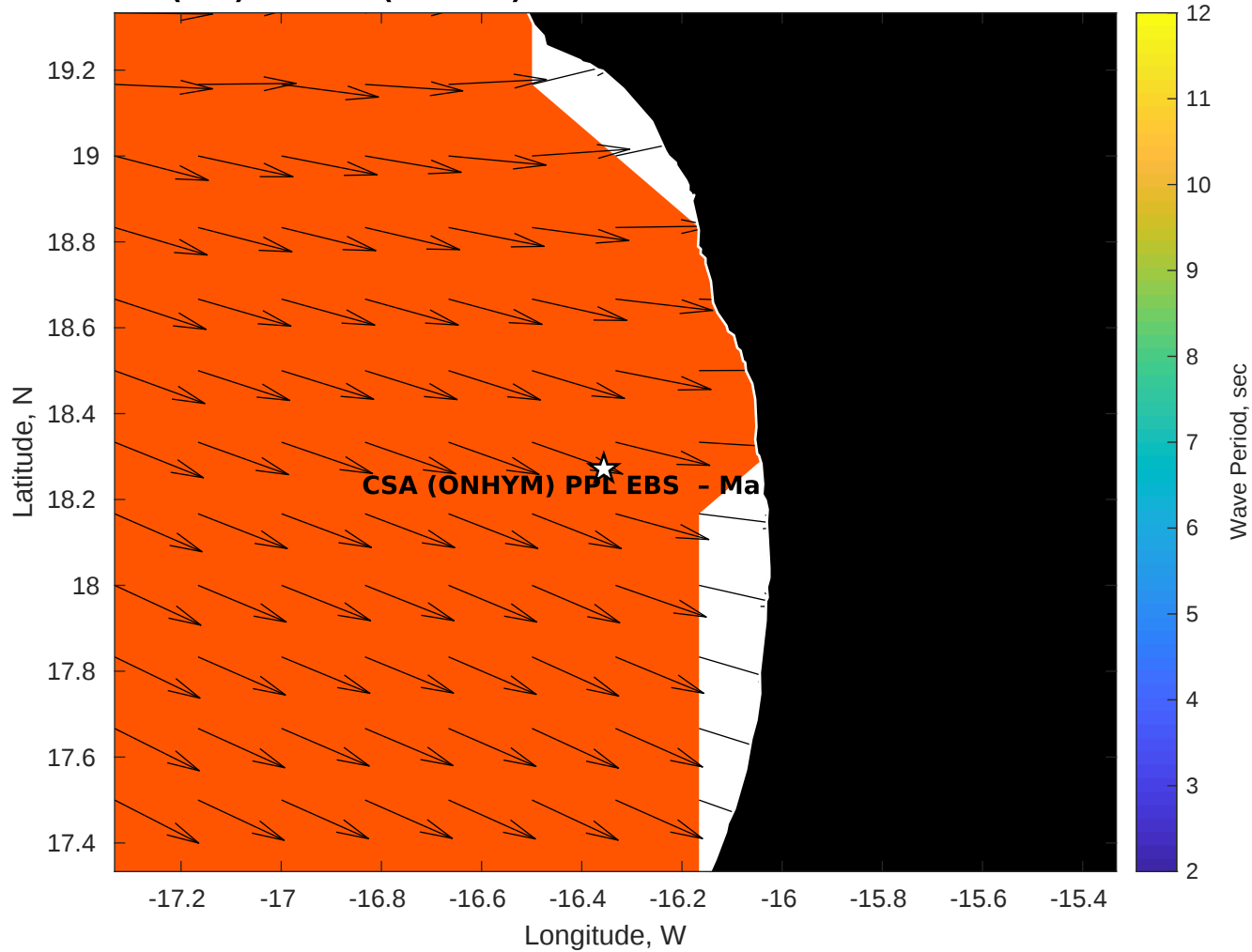
Wave Period (sec) for CSA (ONHYM) PPL EBS - Mauritania at 19-Nov-2025 21:00:00
