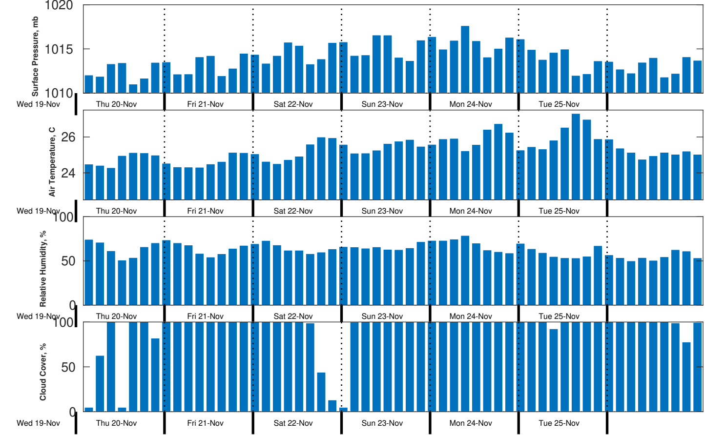
Met Forecast for CSA (ONHYM) PPL EBS - Mauritania from 20-Nov-2025 00:00:00 to 27-Nov-2025 00:00:00
