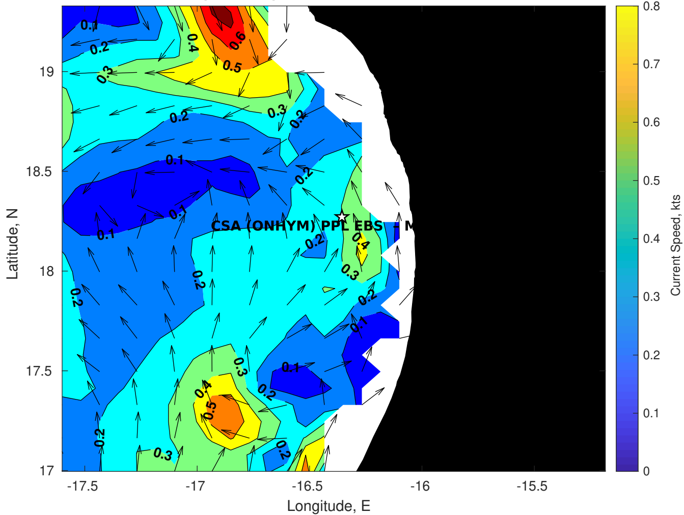
Surface Currents for CSA (ONHYM) PPL EBS - Mauritania at 19-Nov-2025 00:00:00
