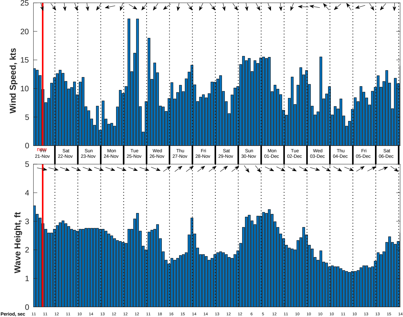
Wind & Wave Forecast for CSA (ONHYM) PPL EBS - Mauritania from 20-Nov-2025 01:00:00 to 06-Dec-2025 01:00:00
