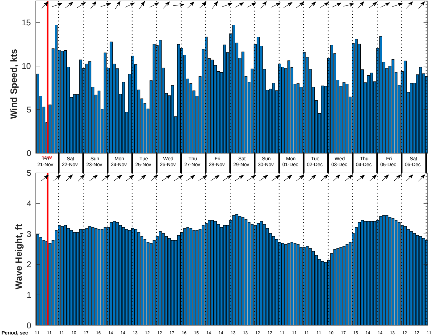
Wind & Wave Forecast for CSA (ONHYM) PPL EBS - Nigeria from 20-Nov-2025 02:00:00 to 06-Dec-2025 02:00:00
