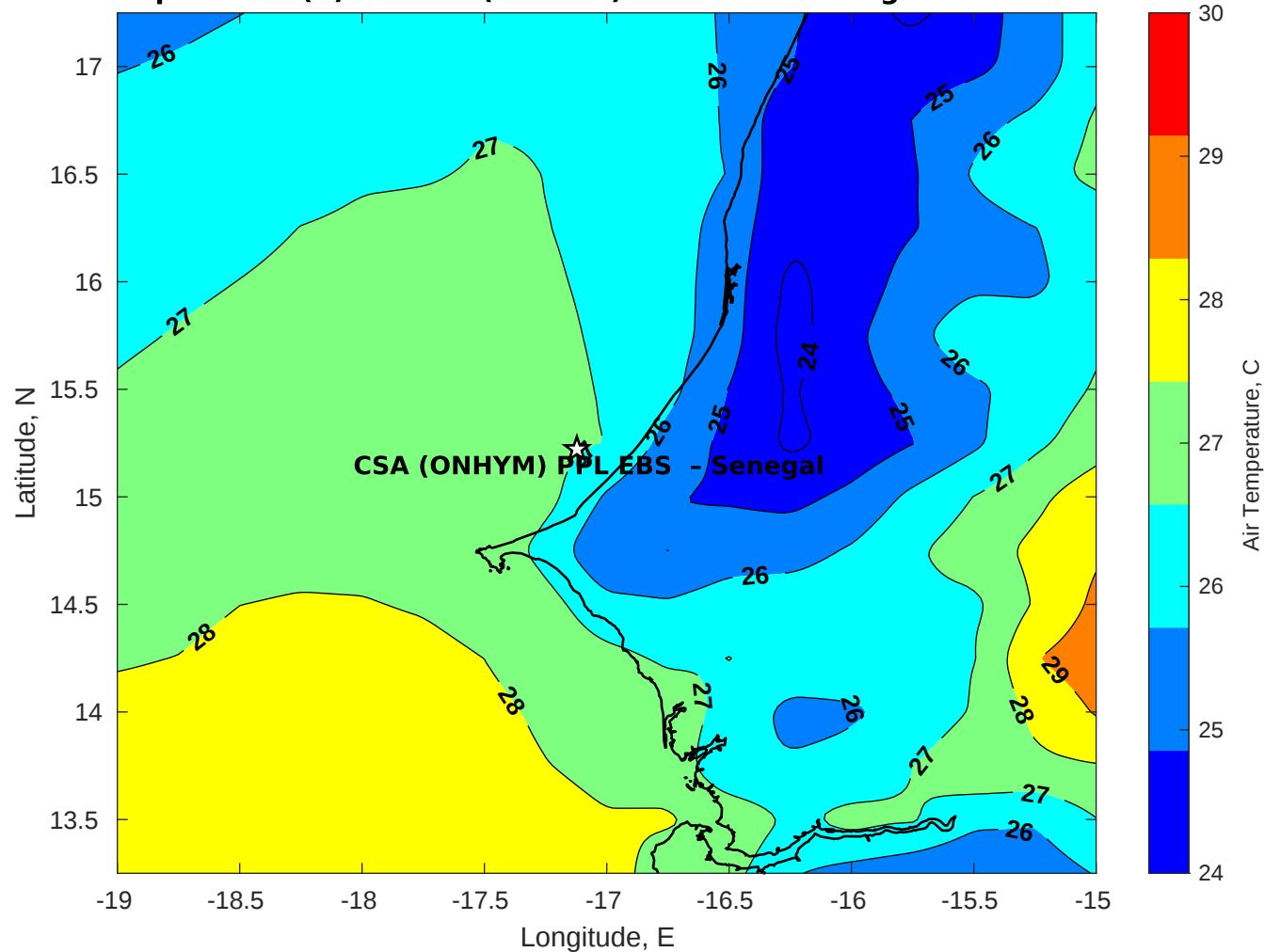
Air Temperature (C) for CSA (ONHYM) PPL EBS - Senegal at 20-Nov-2025
