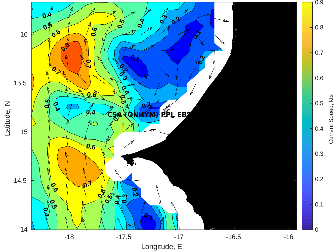
Surface Currents for CSA (ONHYM) PPL EBS - Senegal at 19-Nov-2025 00:00:00
